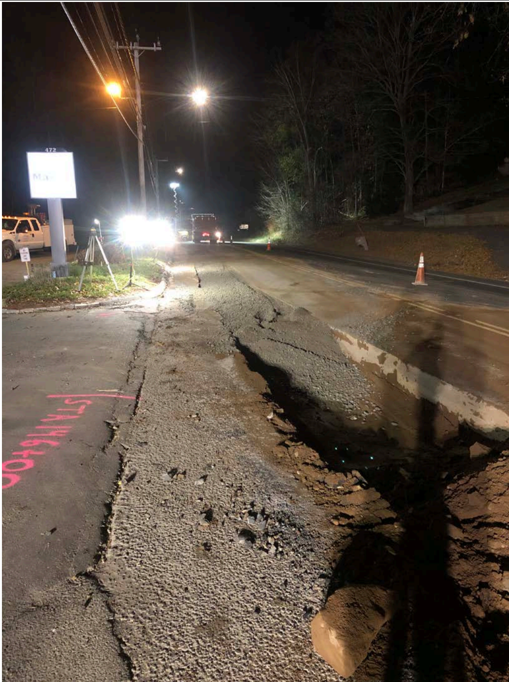
Figure 5 – Processed stone layer above pipe sections 1-3
