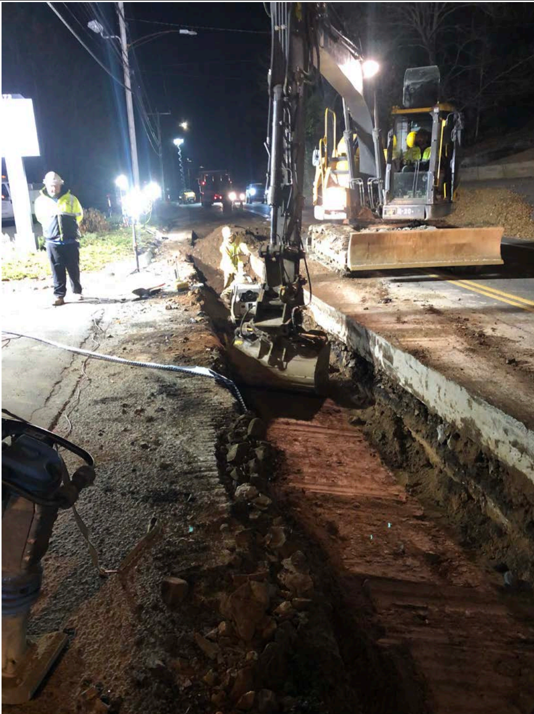
Figure 3 – Spreading, compacting first backfill lift over pipe sections 1-3
