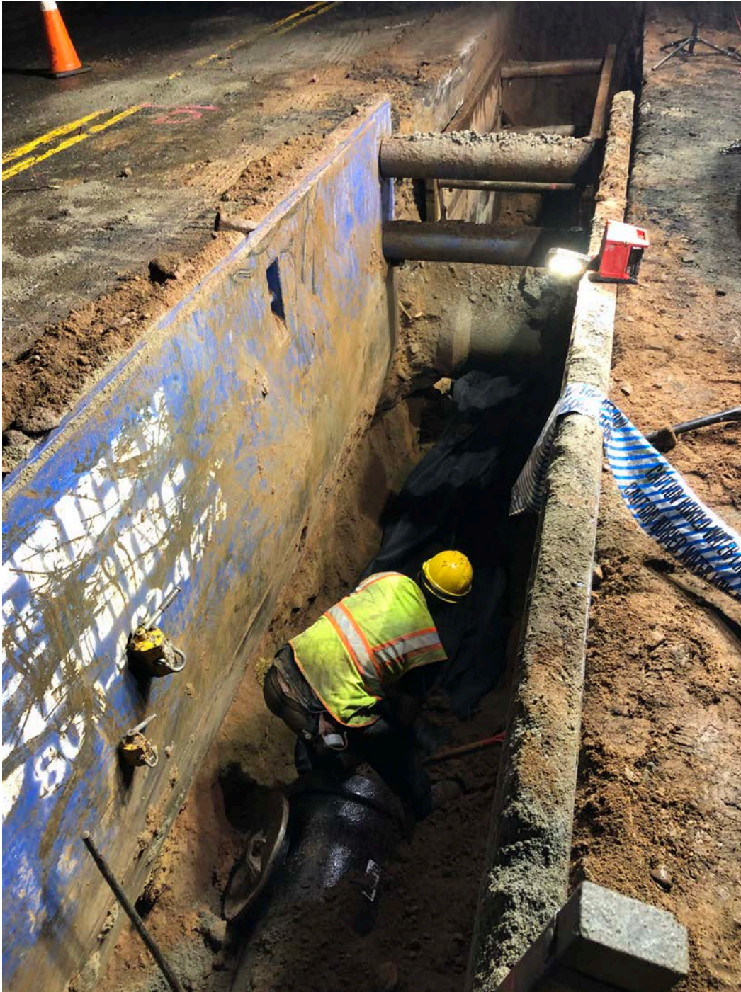
Figure 5 – 5 th pipe section placed, trying to determine if 6 th section will fit under storm drain at Sta. 137+65
