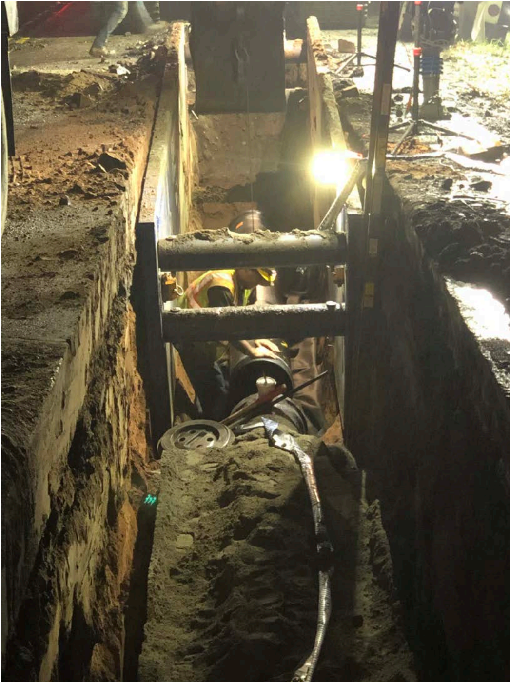
Figure 3 – Placing 3 rd pipe section
