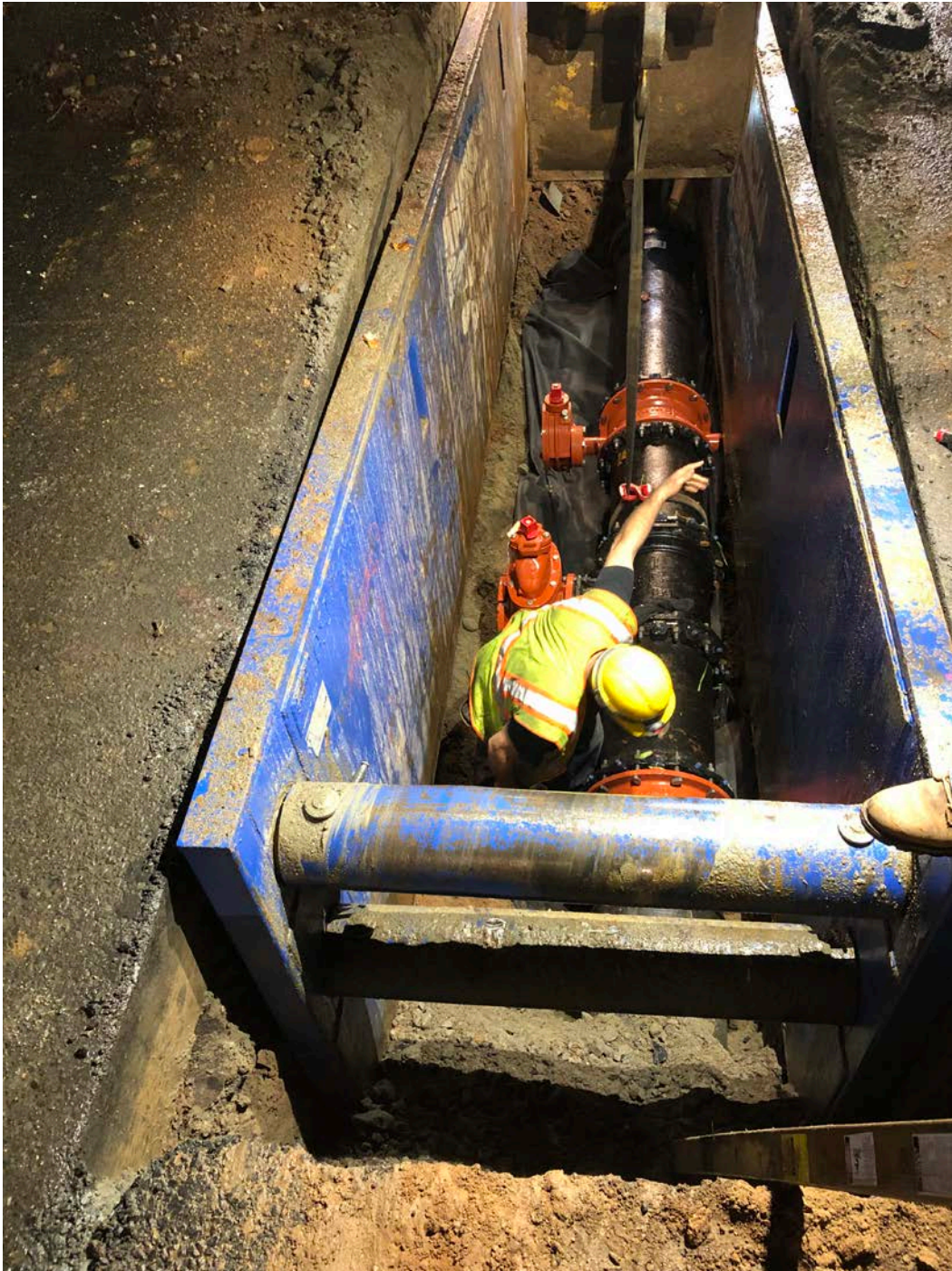
Figure 1 – Placing first valve section at Sta. 136+58 (Royal Oak Drive)
