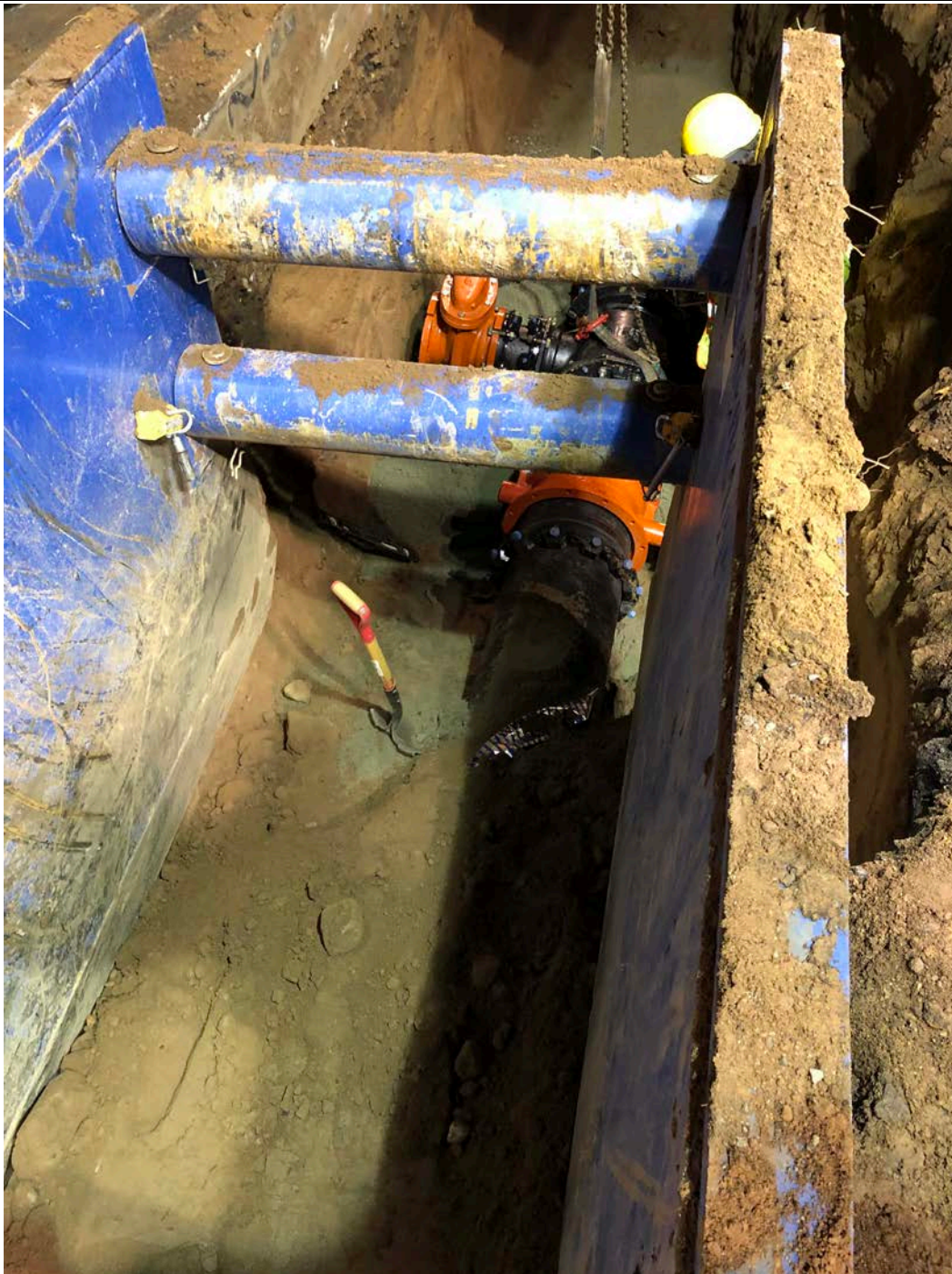
Figure 6 – Valve section in place at Sta. 132+30
