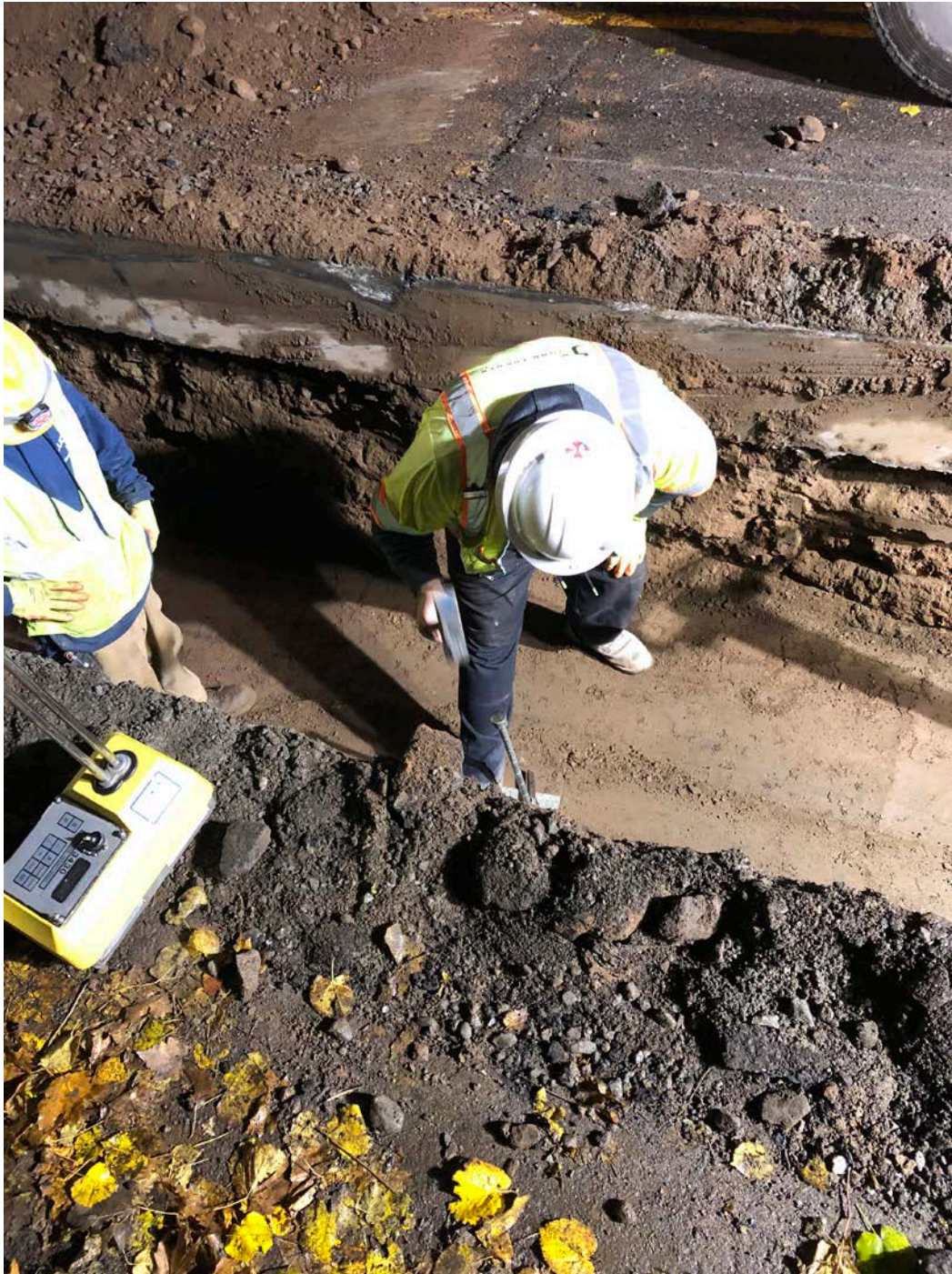
Figure 4 – Compaction testing 2 nd fill lift over section 2
