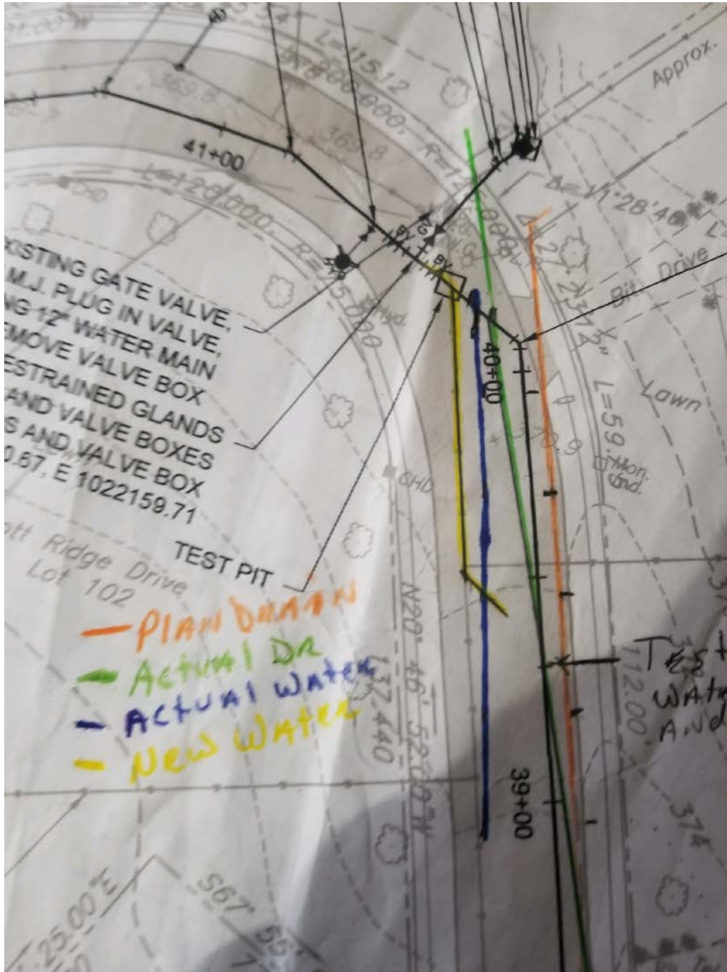
Figure 1 – Plan showing changes. Orange line is the expected drain location. Green is the actual drain location. Blue is the actual location of the existing 12” water main. Yellow is the revised 16” DI Line.
