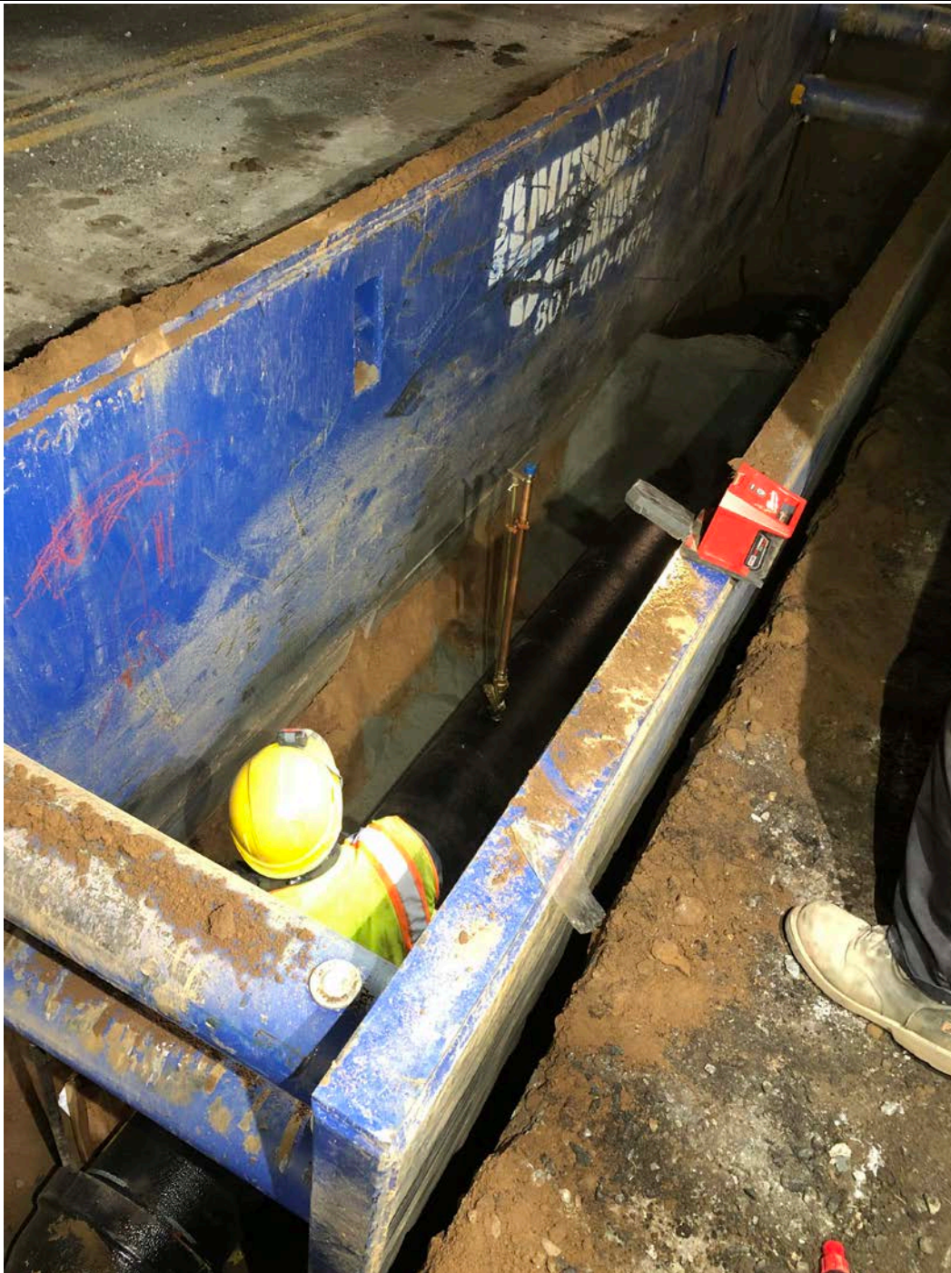
Figure 5 – Air release valve being assembled at Sta. 130+60
