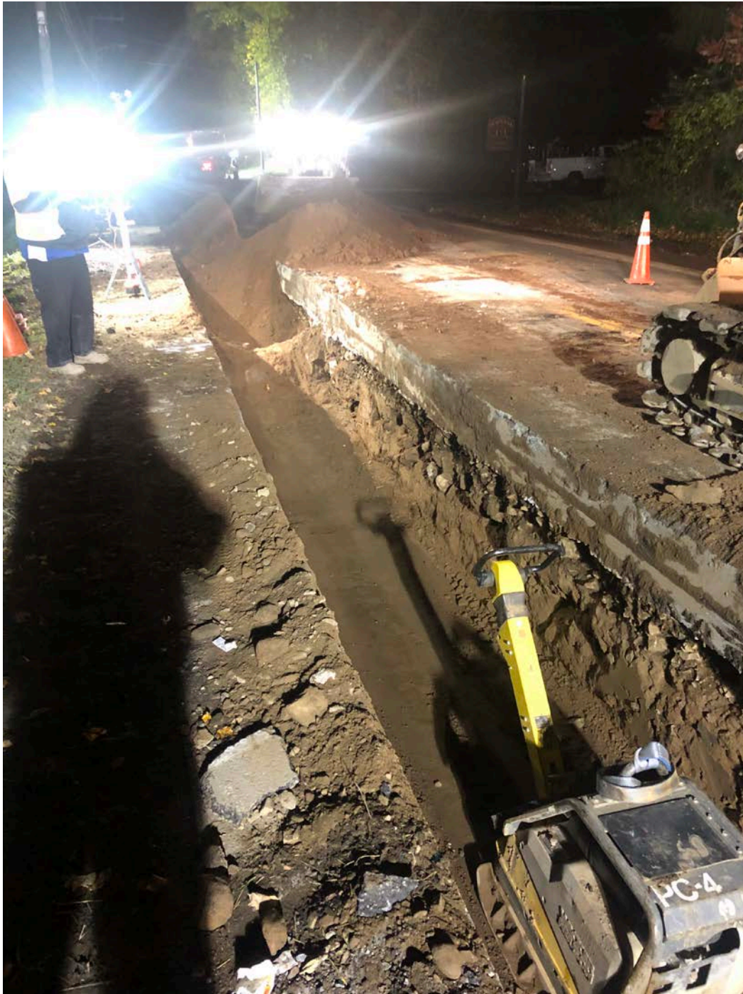
Figure 6 – Compacted 2 nd backfill lift above sections 2-3
