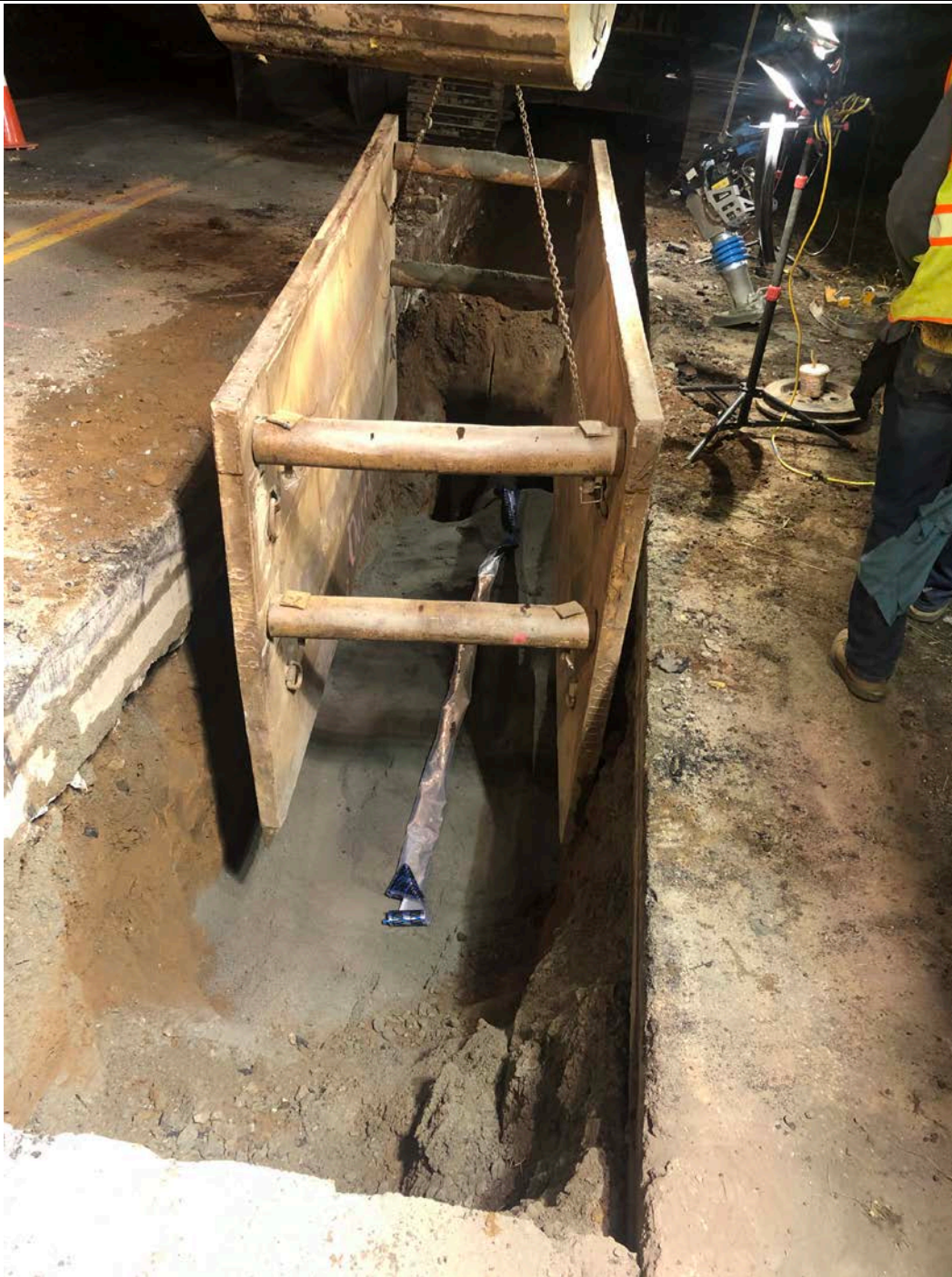
Figure 2 –First pipe in at Sta. 126+74, covered with bedding and warning tape
