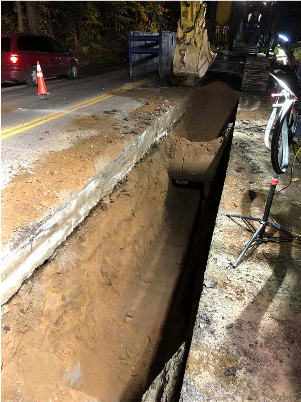
Figure 1 – Storm drain (32" RCP) at Sta. 127+12
