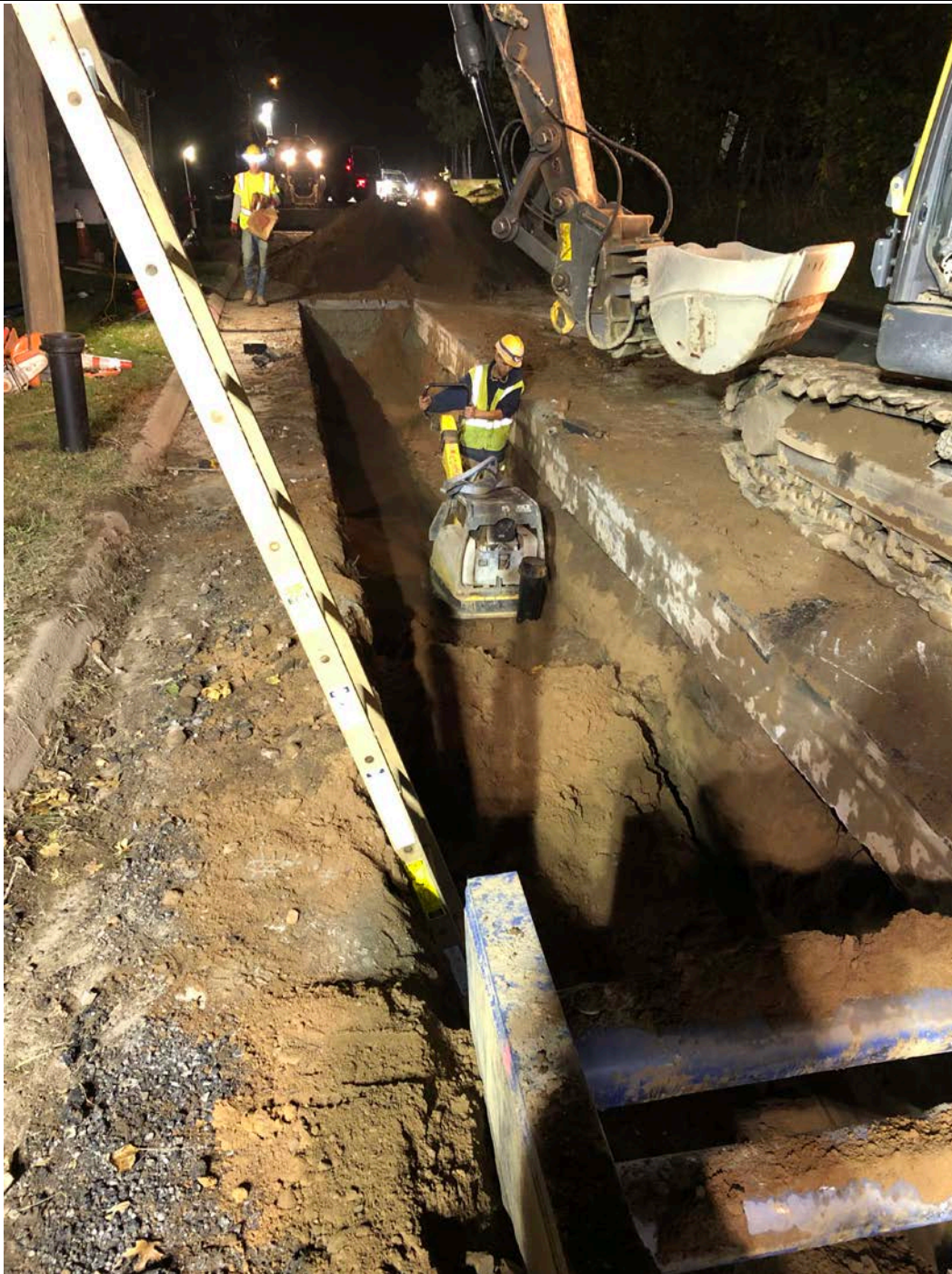
Figure 5 – Compacting fill over Tee section
