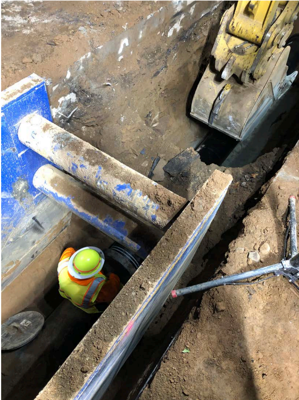
Figure 6 – Attaching 6 th pipe section, feeding underneath storm drain at Sta. 125+80
