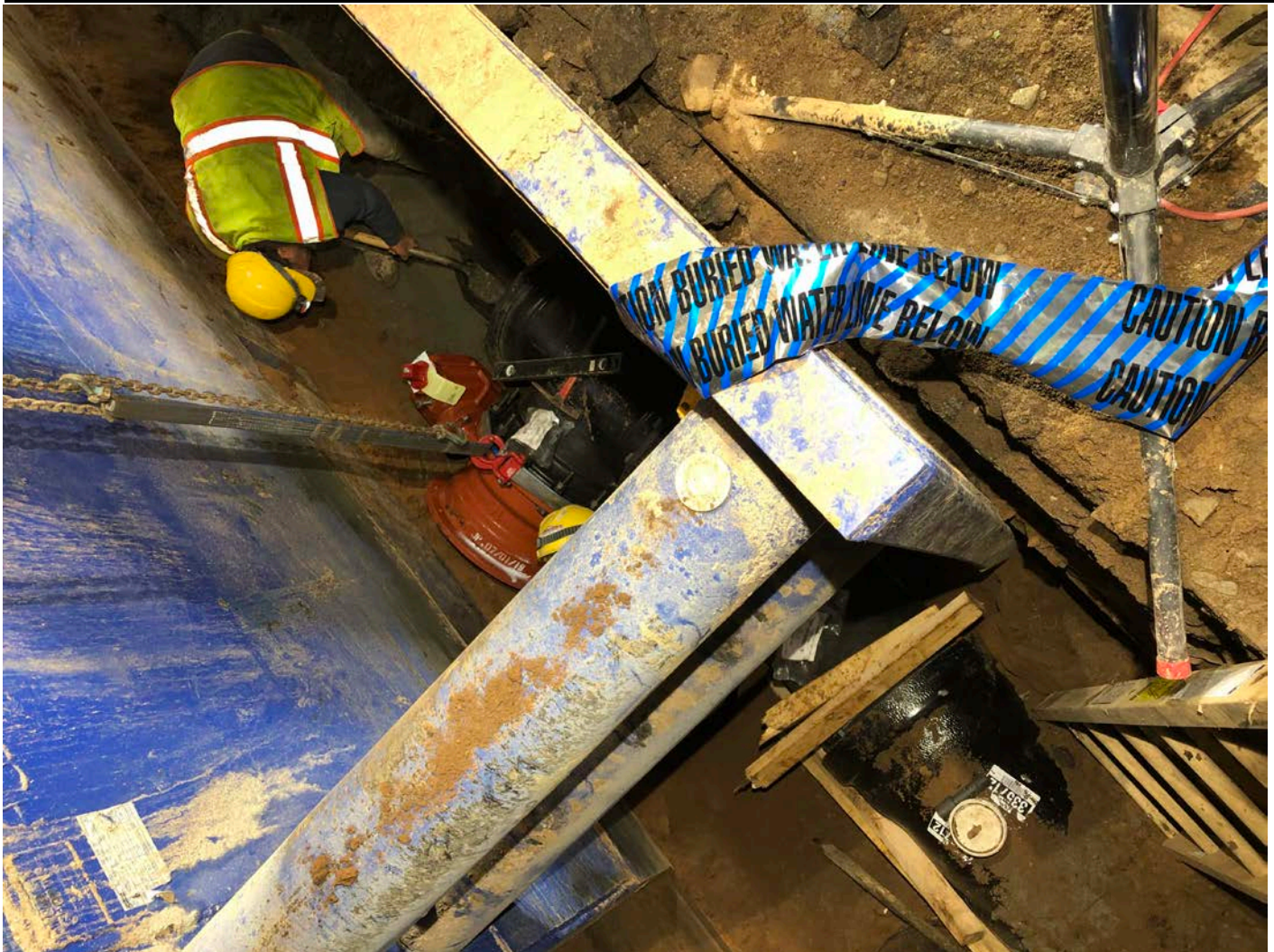
Figure 3 – Attaching Tee section at Sta. 125+20 (connection to water meter vault)
