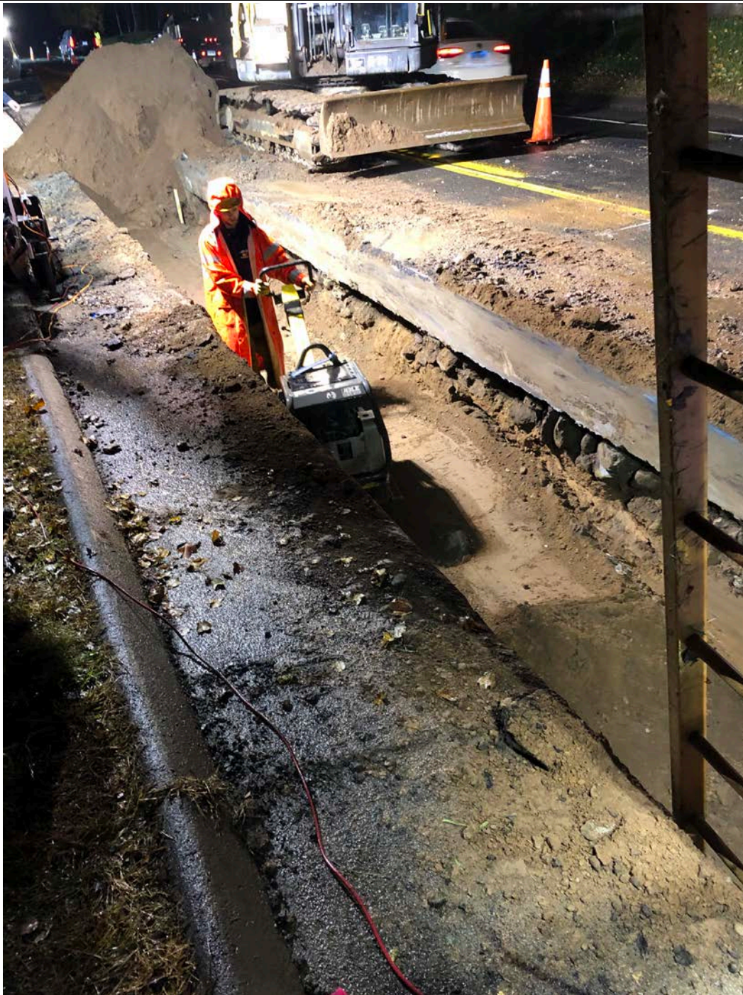
Figure 2 –Plate compacting over 1 st -2 nd pipe sections
