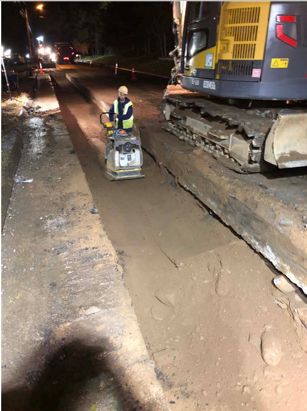
Figure 6 – Compacting 2 nd lift above 1 st -6 th sections
