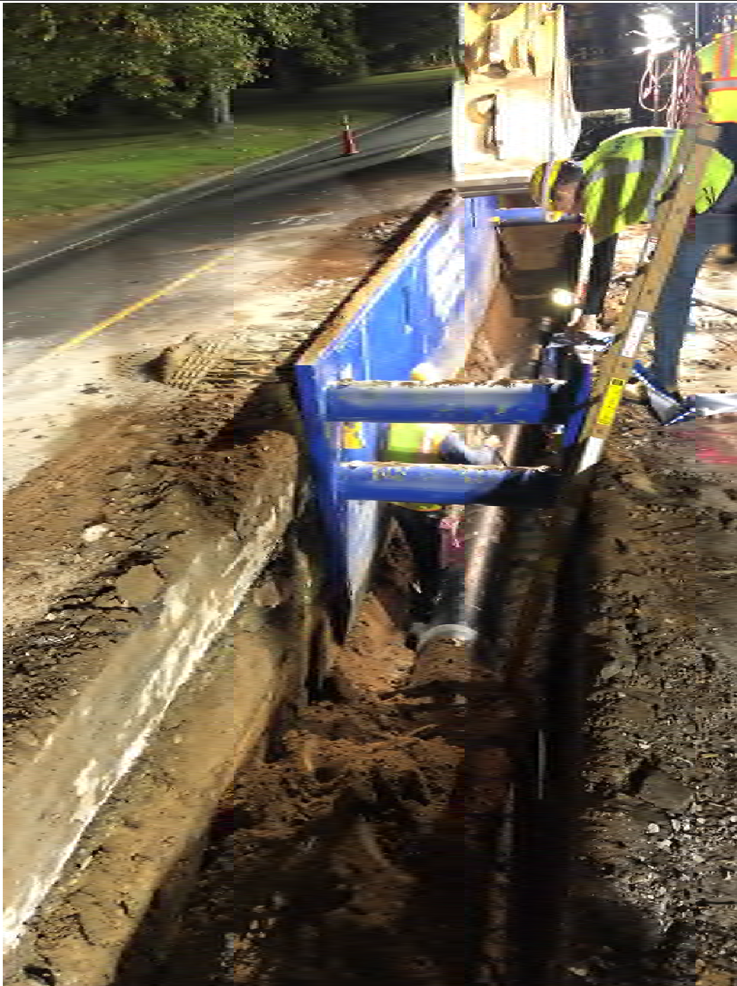
Figure 7 – Attaching 7 th pipe section
