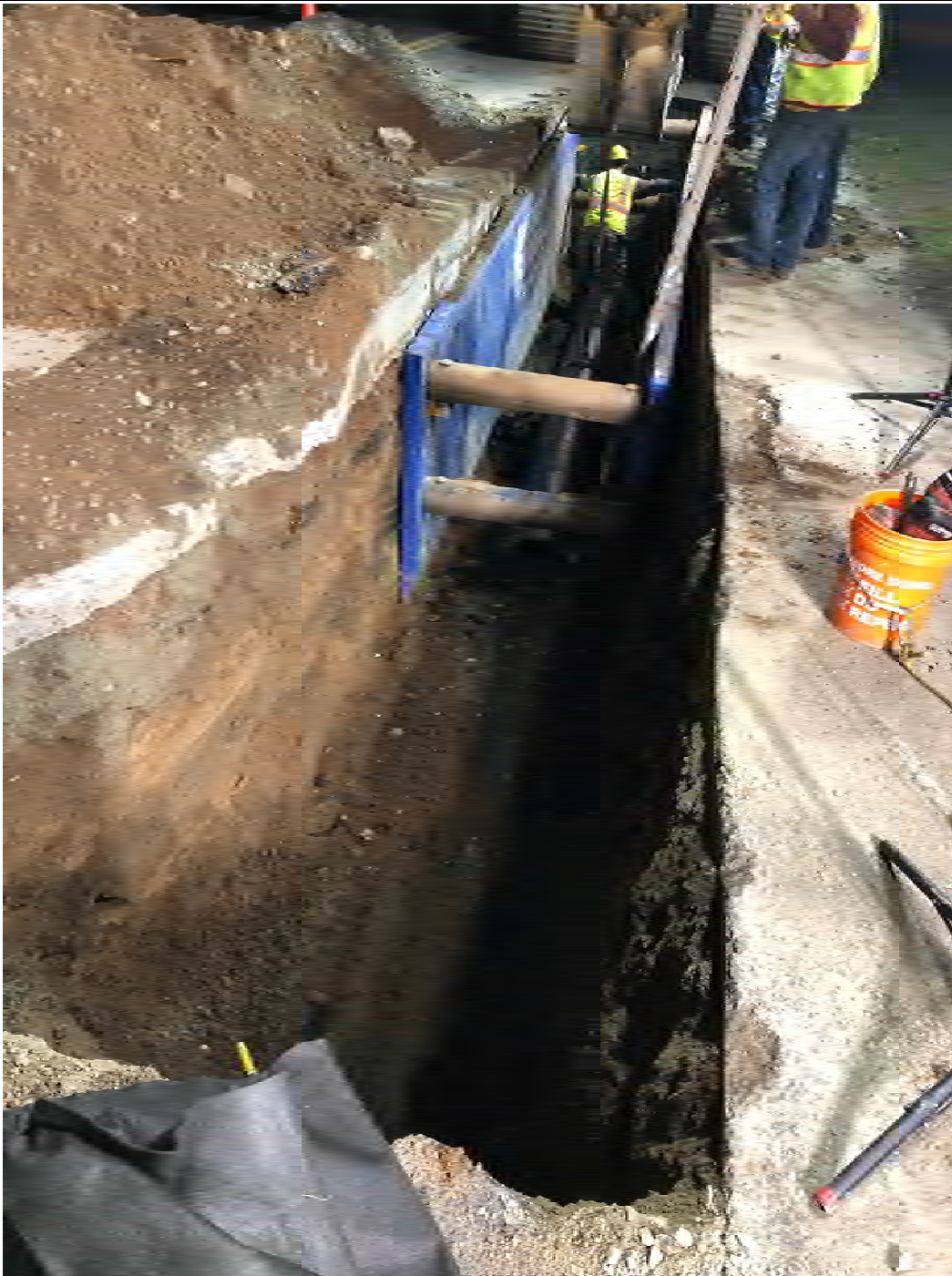
Figure 1 – Lowering first pipe section to attach to pipe at Station 100+46
