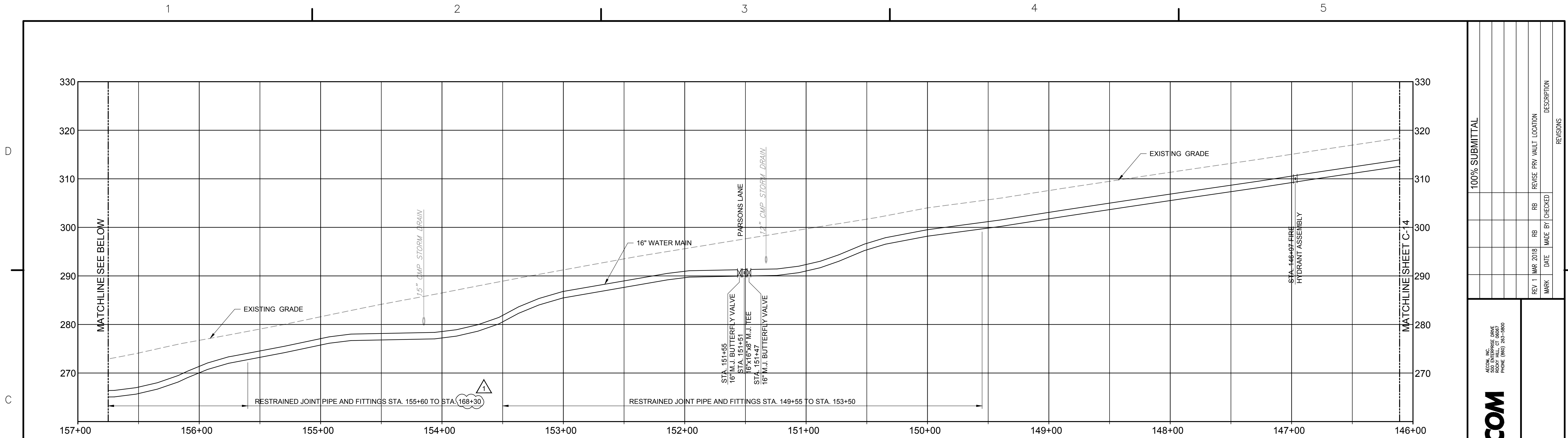
MAIN STREET (ROUTE 17) PROFILE STA. 146+11 TO STA. 156+75
