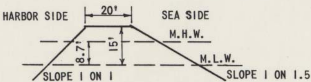
SECTION OF BREAKWATER
