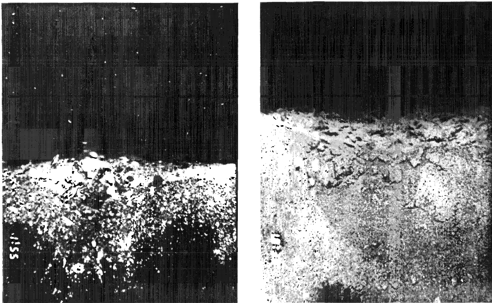
Figure 3-8. REMOTS® photographs of reference area stations WREF (200E) and NLON (200E). The WREF site was characterized by scoured shell lag deposits and fine sands. The successional stage at this reference area station was indeterminate. Sediment grain size major mode at NLON-REF consisted of very fine sands (4-3) phi. An intact tube mat formed by tubicolous amphipods or Stage II organisms characterized the sediment surface of NLON-REF station 200E.
