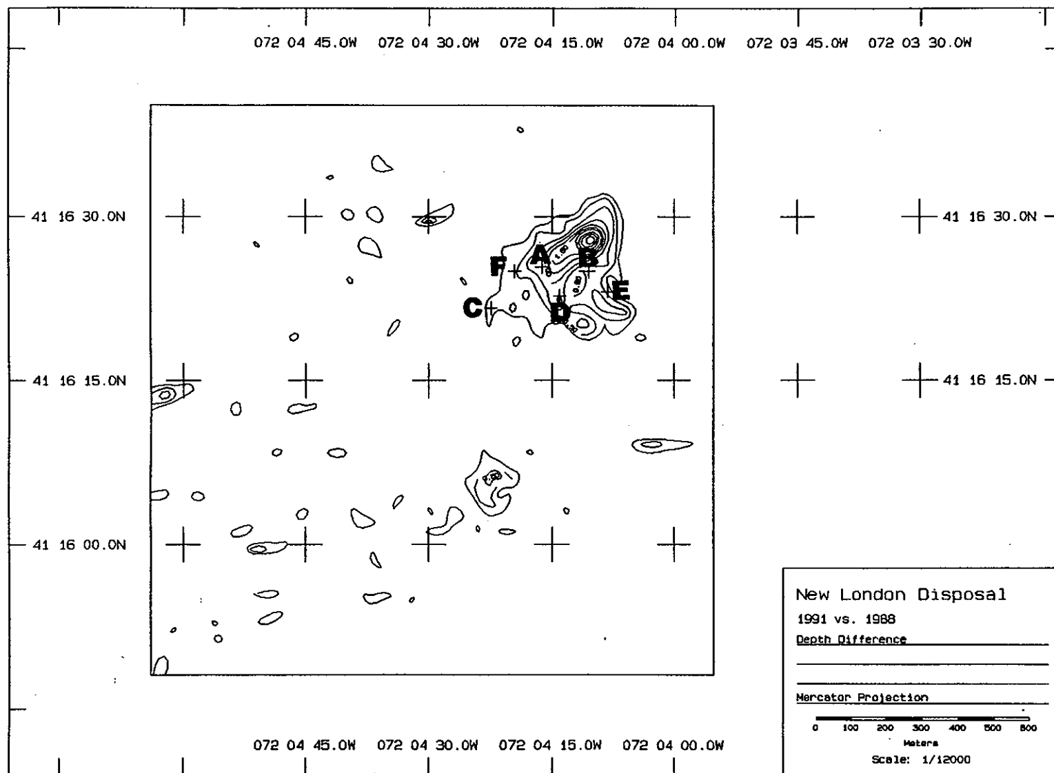
Figure 4-1. Contour plot of volumetric differences between October 1988 (prior to capping) and June 1991, showing locations of the LORAN-C disposal points
