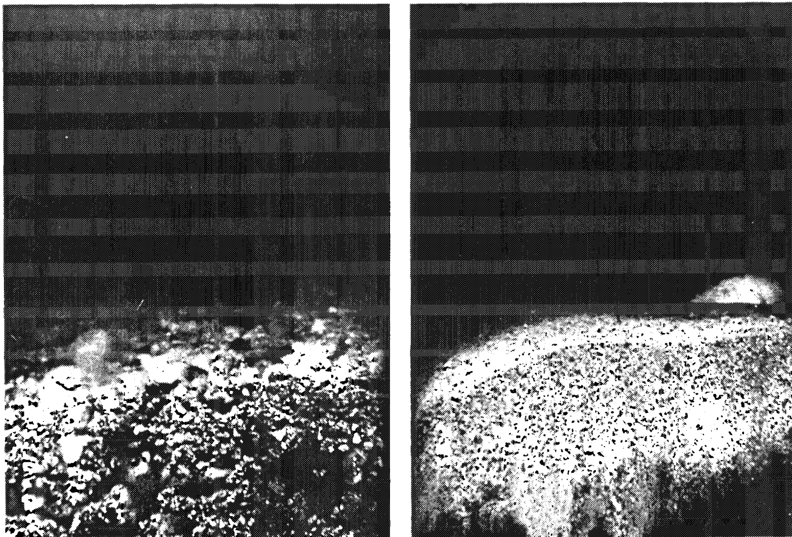
Figure 3-7. REMOTS® photographs of disposal site Stations 100SE (left) and 200E (right). Station 100SE sediments consisted of cobble, gravel, and coarse sands. Coarse sands were also present at stations with active bedforms such as 200E.
