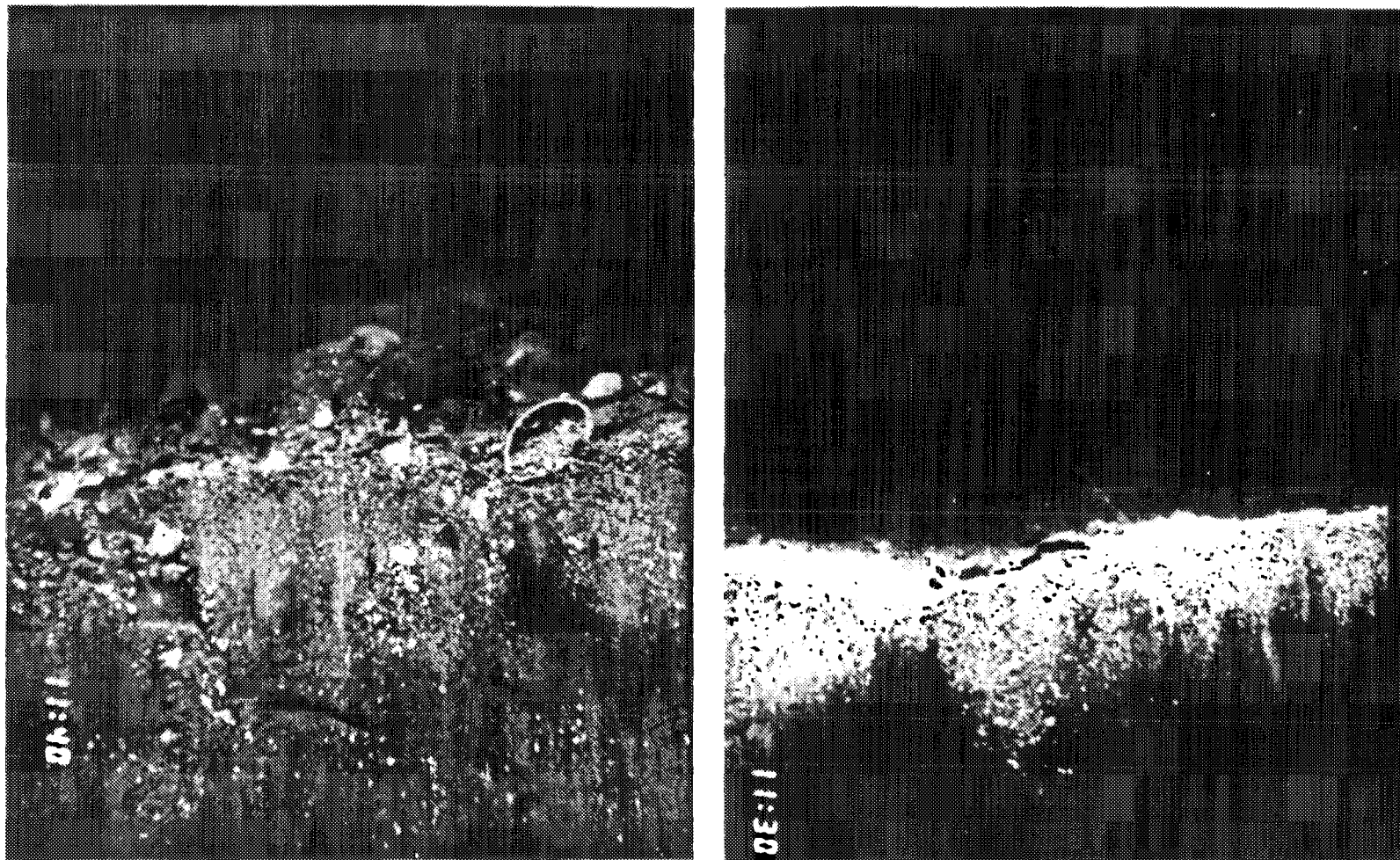
Figure 3-13. REMOTS® photographs of fresh dredged material at 200S (left) and 300S (right). The surface of Station 200S consisted of shellhash and mud clasts while 300S showed a large difference of optical reflectance between the sands (high reflectance) and underlying mud (low reflectance). This station also showed the presence of bedforms and washing of fine sediments by bottom currents from the sediment surface layer.
