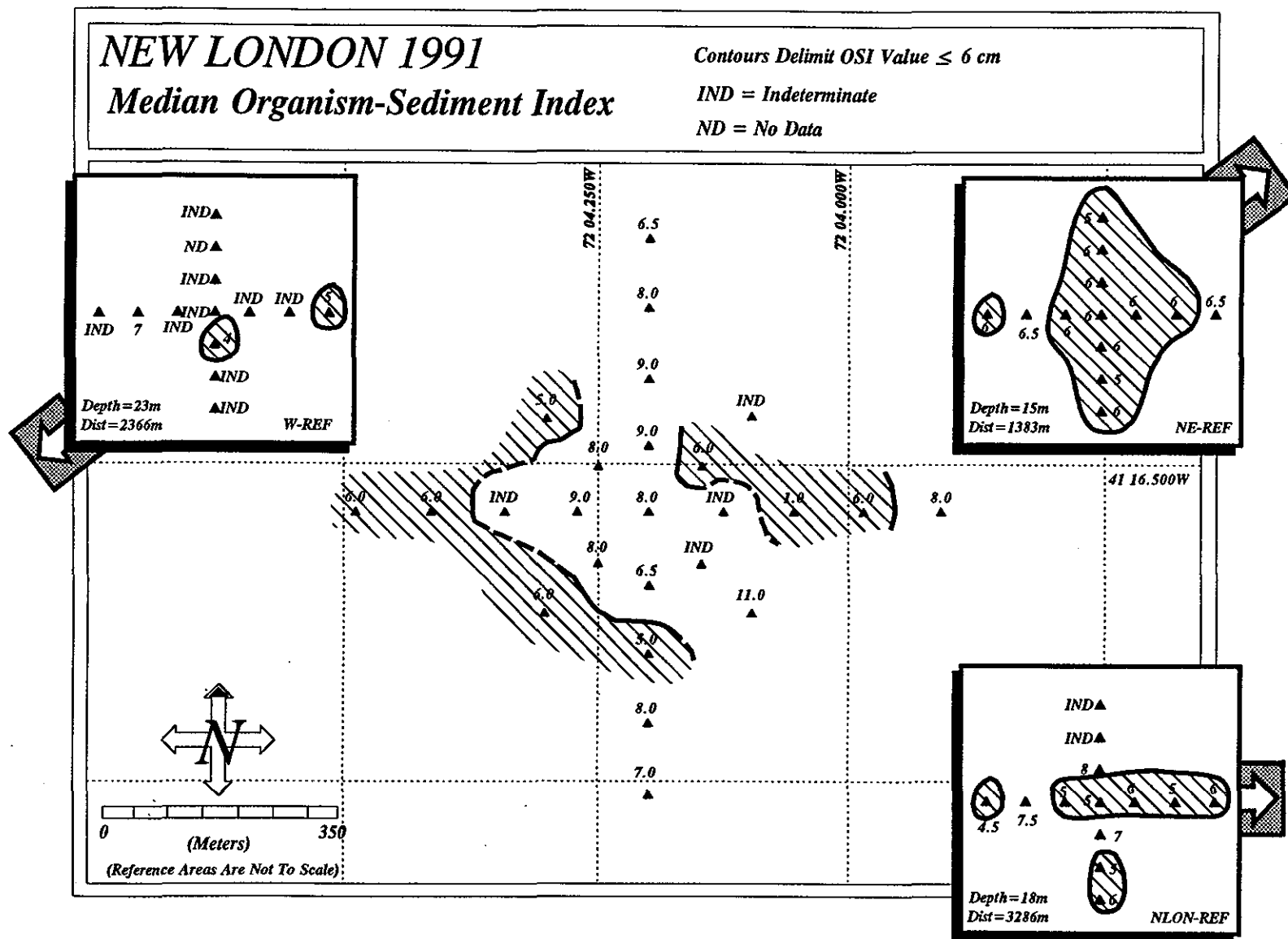
Figure 3-19. Spatial distribution map of median Organism-Sediment Index (OSI) values at the New London Disposal Site and reference stations. Distances are measured from the disposal site center to the respective reference area center.
