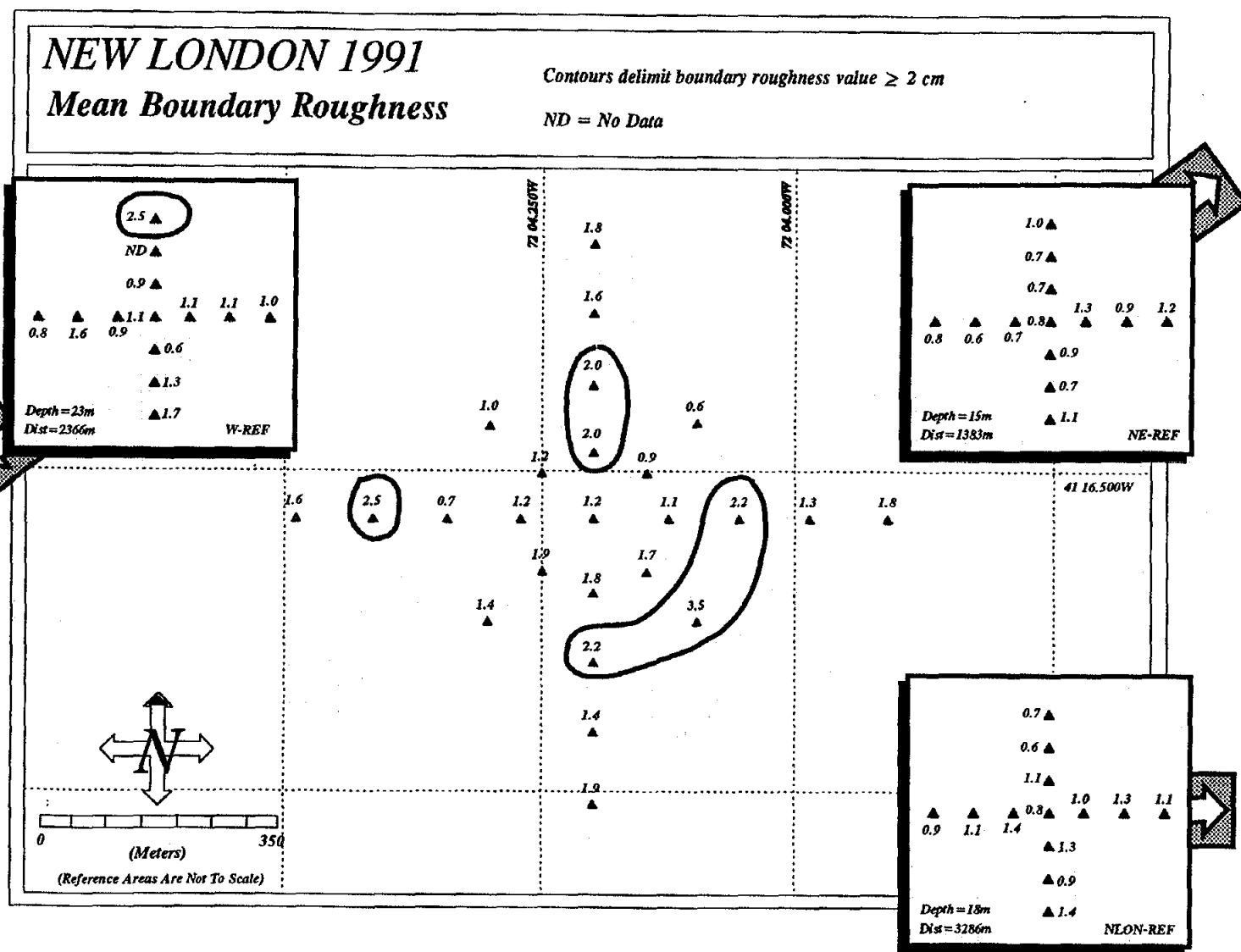
Figure 3-10. Spatial distribution of mean boundary roughness values at the pooled disposal site and reference stations. Distances are measured from the disposal site center to the respective reference area center.
