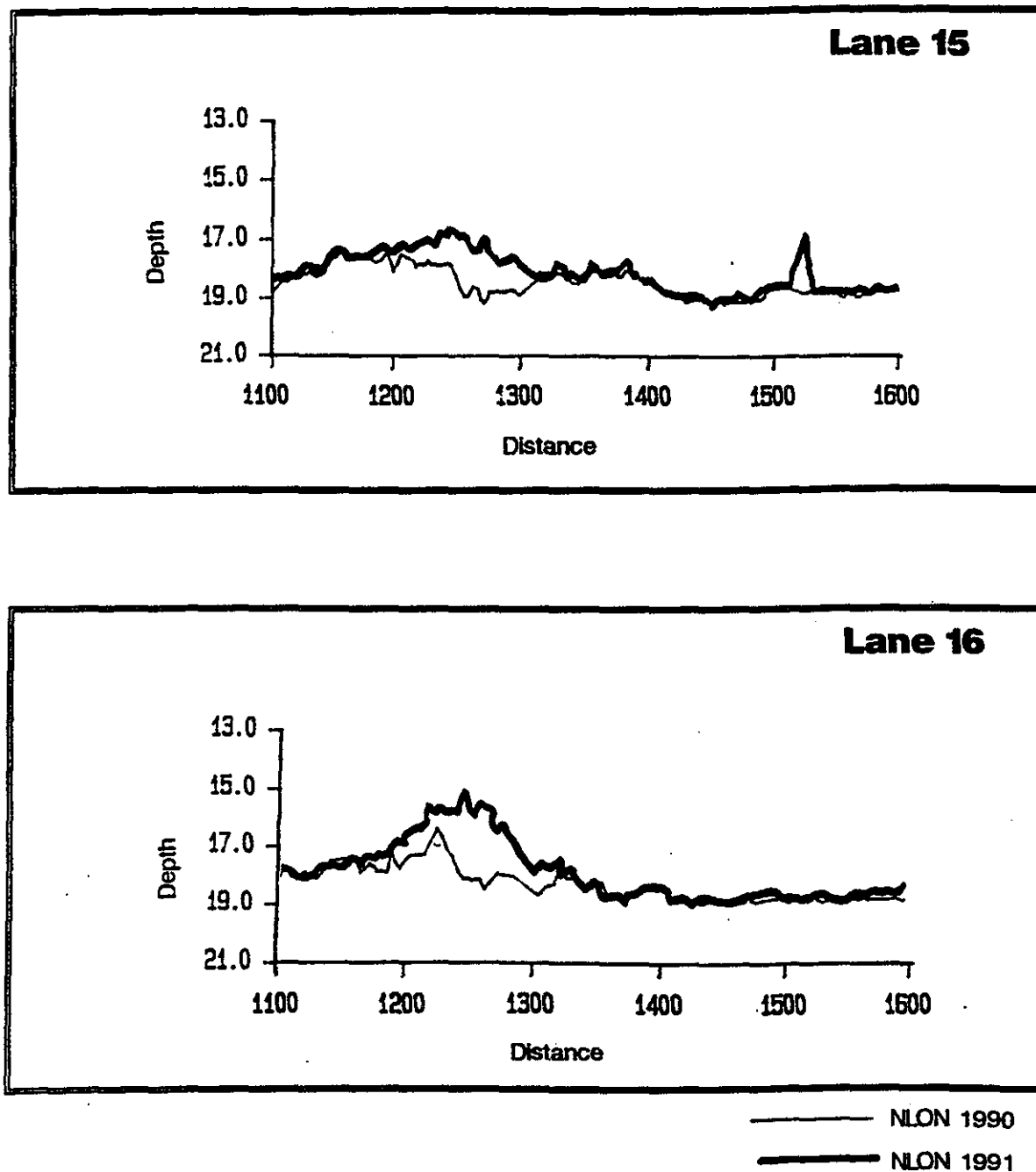
Figure 3-5. Depth profile plots of bathymetric survey lanes 15 and 16 which transect the NL-TR mound. The depth profile plot of lane 16 indicates a maximum change in height at the mound of 3 m.
