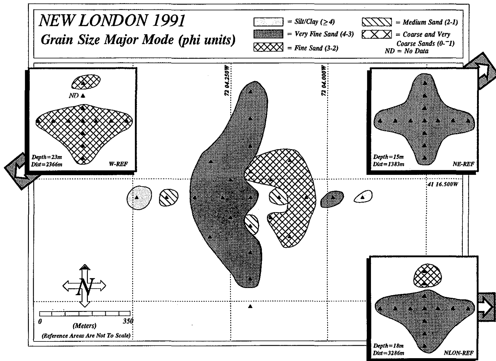
Figure 3-6. Distribution map of grain size major mode at the New London Disposal Site and reference areas. Distances are measured from the disposal site center to the respective reference area center.
