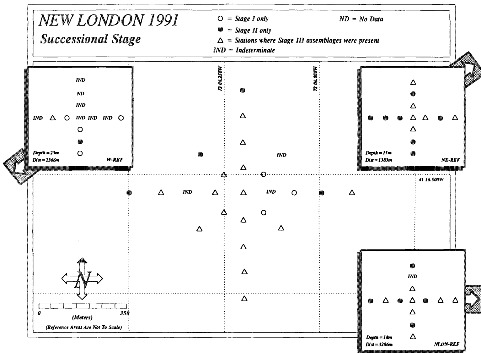
Figure 3-17. Spatial distribution of successional stages at the New London Disposal Site and reference stations. Distances are measured from the disposal site center to the respective reference area center.
