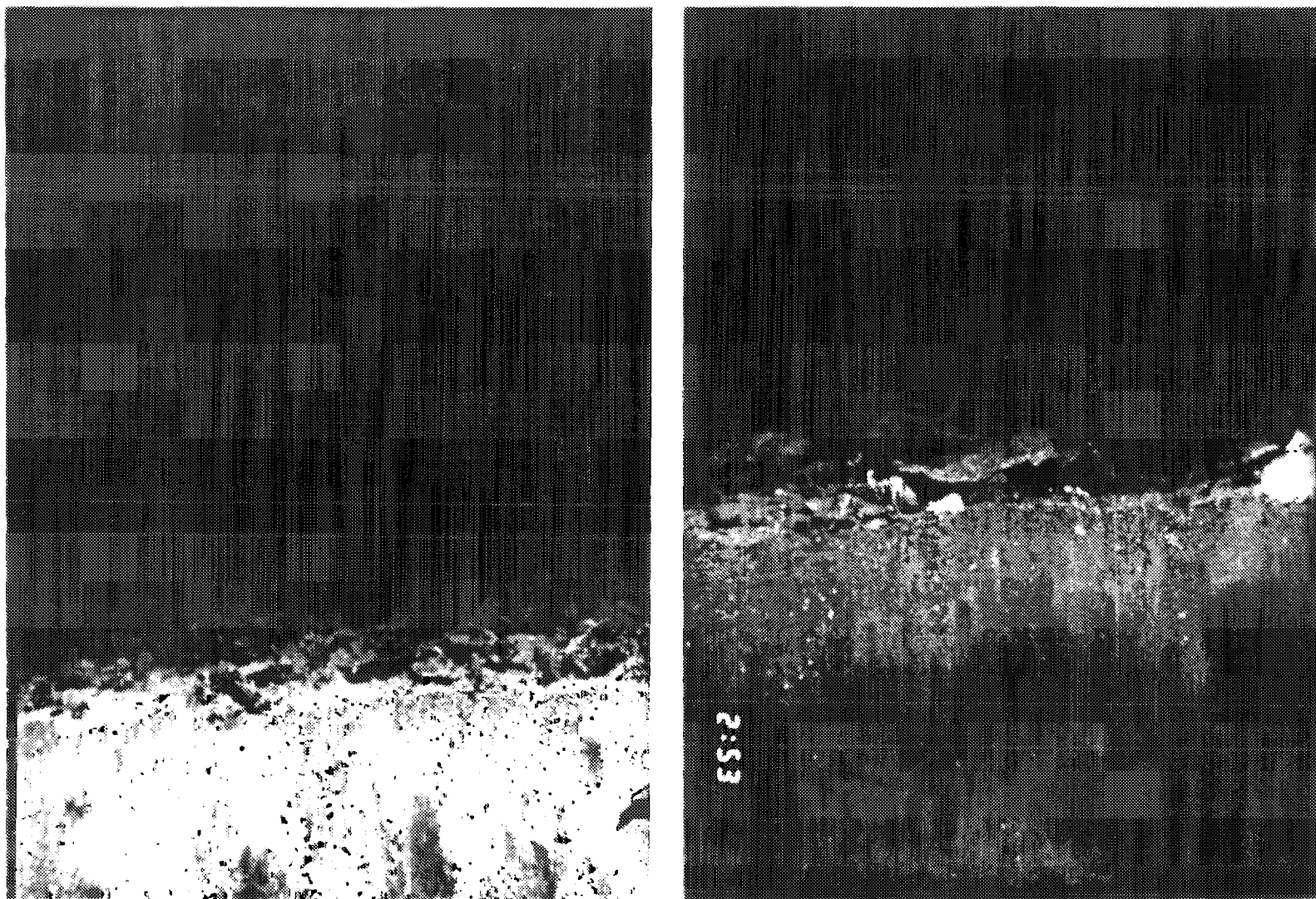
Figure 3-18. REMOTS® photographs from disposal site stations 300N (left) and 200SW (right). The successional stages present at these stations, Stage II on Stage III (300N; left) and Stage III (200SW; right) typified the majority of stations on the site.
