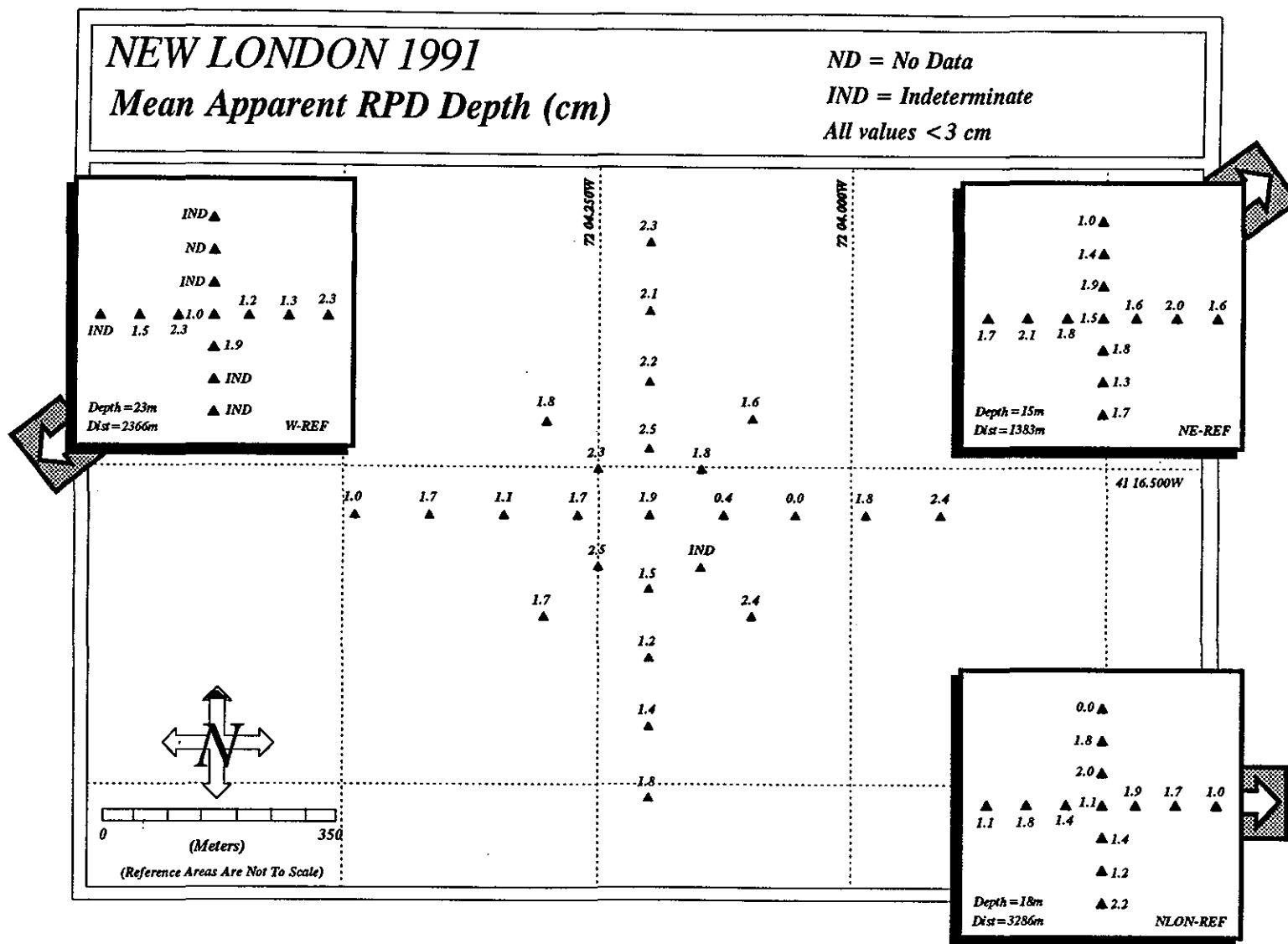
Figure 3-16. Spatial distribution of mean apparent RPD depths at the New London Disposal Site and reference area stations
