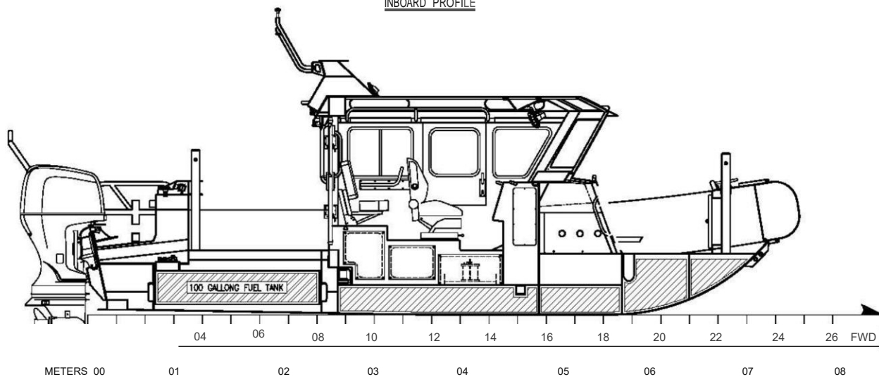
OUTBOARD PROFILE
