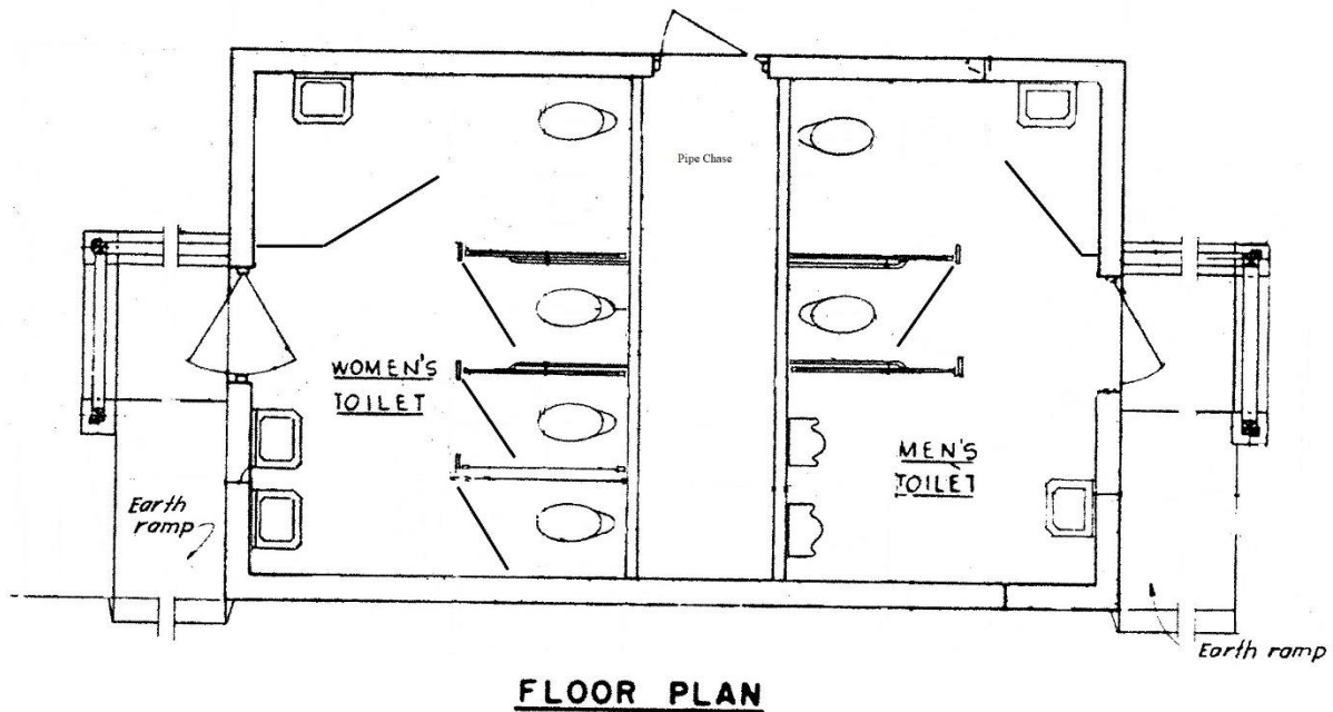
Exhibit 5: Approximate floor layout of the Elm Brook Park upper restroom building. The water tank and pipe (not shown in diagram) are located in the back half of the pipe chase opposite the door. Space is limited in this pipe chase.
