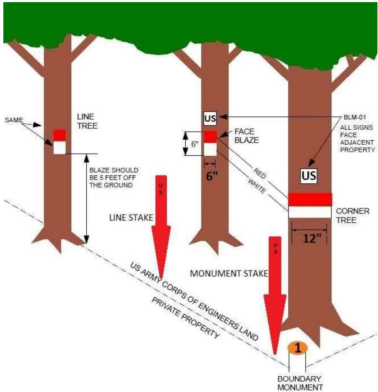
FIGURE NO 2: Boundary Marking Specifications
