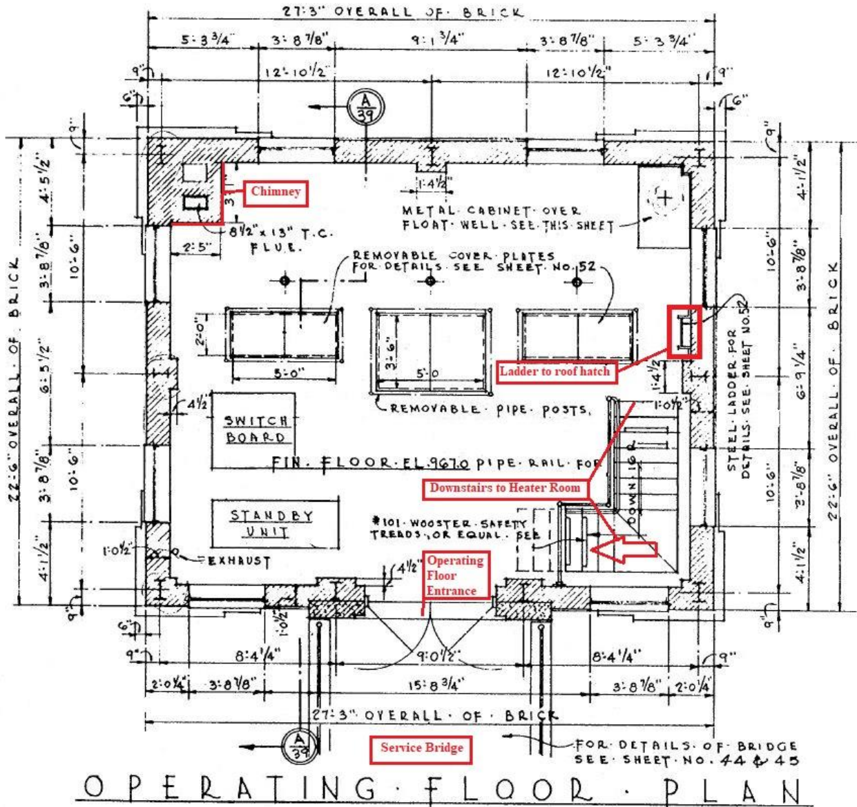
Exhibit H – Operating Floor Plan showing chimney location, stairs to Heater Room Floor, and fixed ladder to access the Roof; Not to Scale.
