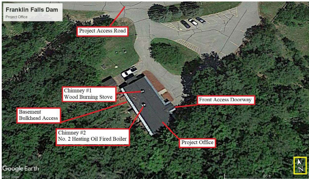
Exhibit B: Franklin Falls Project Office Overview
