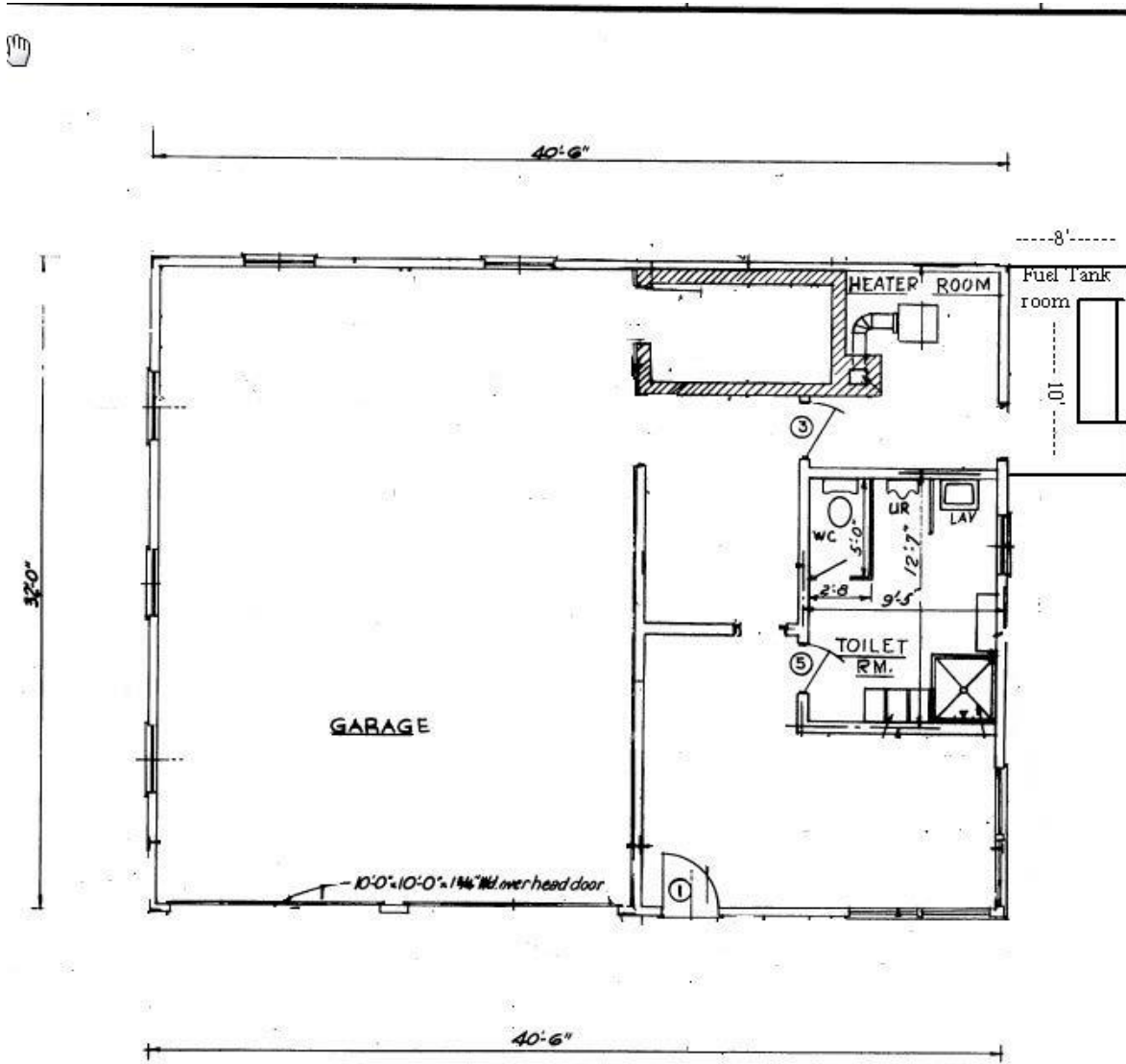
FLOOR PLAN
