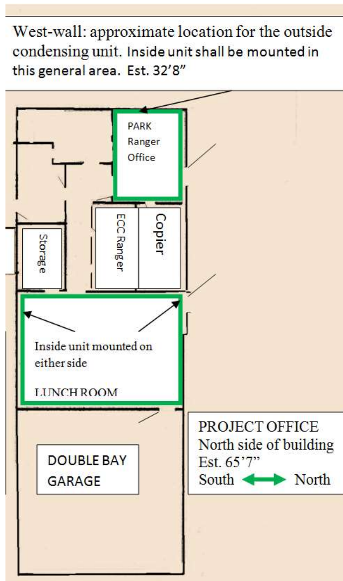
Exhibit B: Interior layout of the building. The rooms outlined in green are the two spaces where the interior heads shall be installed.
