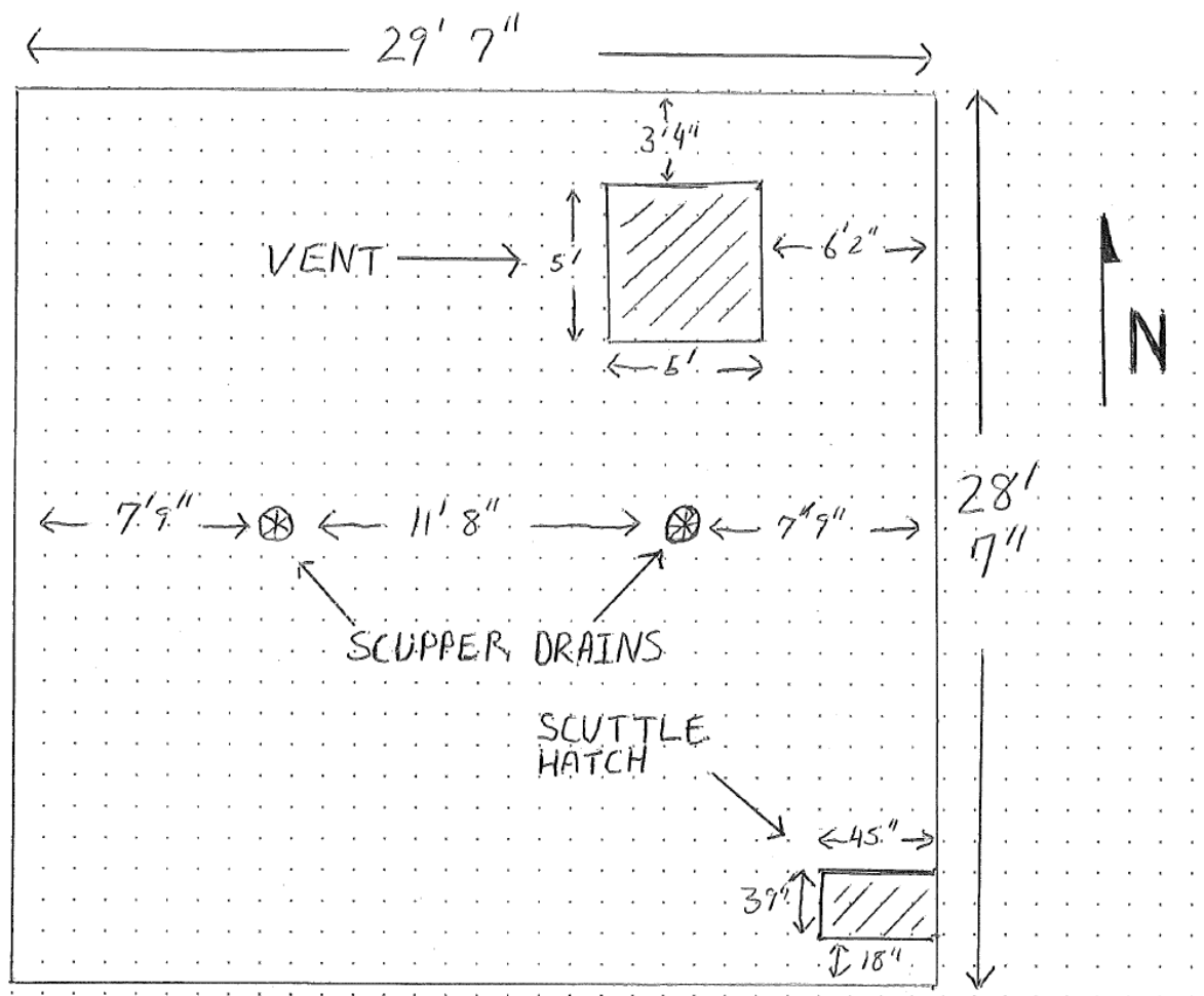
Sketch 1: Diagram of North Springfield Dam Gatehouse roof. showing the original roof dimensions 27' 7" x 29' 7".
