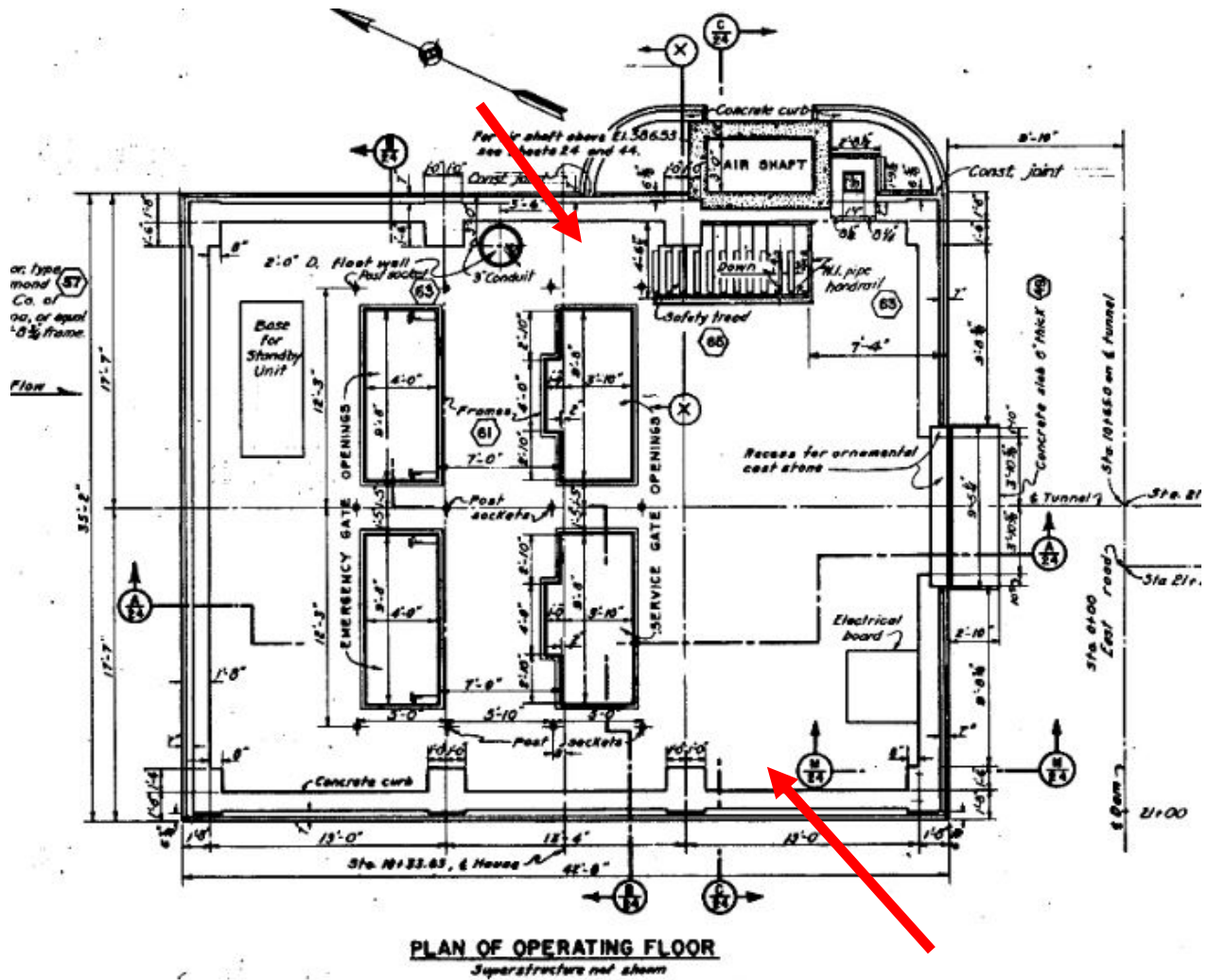
Informational Photo 6: Plan of the operating floor. “Upper” floor plan. Red arrows depict approximate locations for new heating ducts and floor grates.
