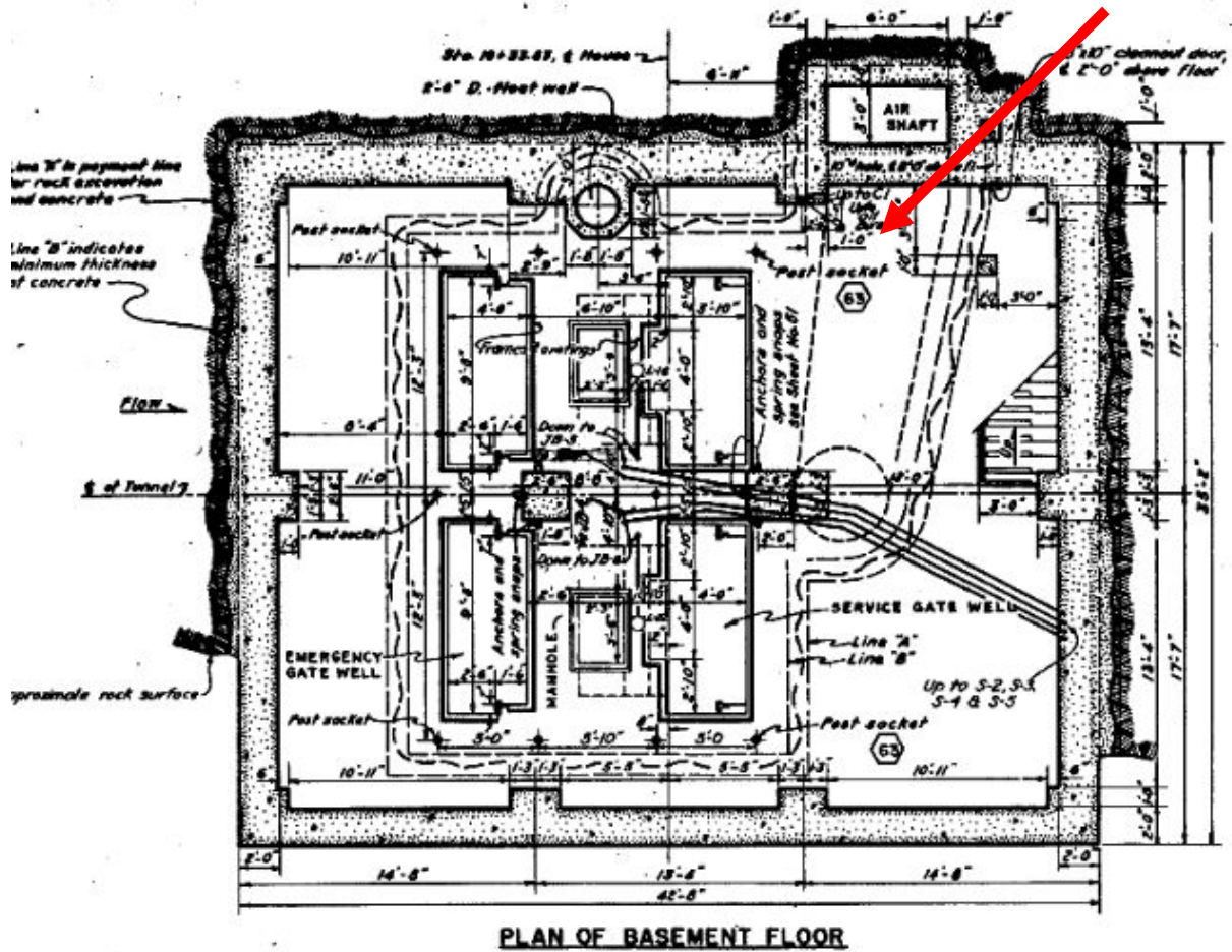
Informational Photo 7: Plan of the basement floor. "Lower" floor plan. Red arrow depicts the approximate location for the new oil fired hot air furnace.
