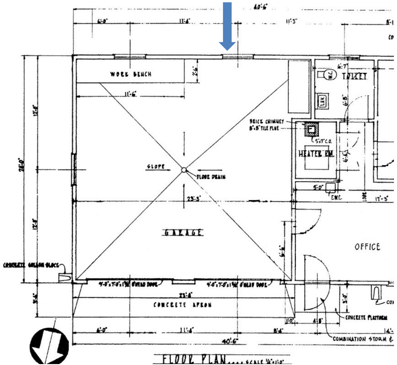
Exhibit I: Everett Dam Project Office floor plan with blue arrow pointing at “warm bay” garages.
