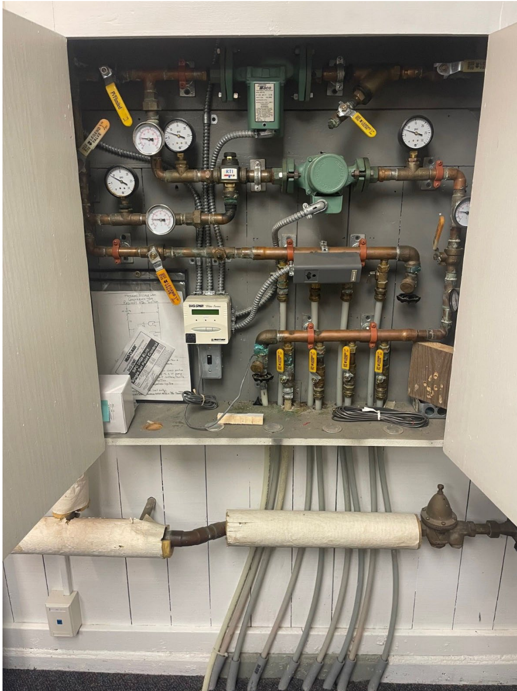
Image of slab heating control system and thermostat
