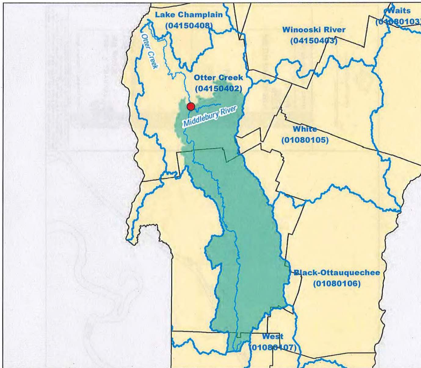
Fig. 11: DU-VT ILF Program 3 Mile Bridge Road Watershed
