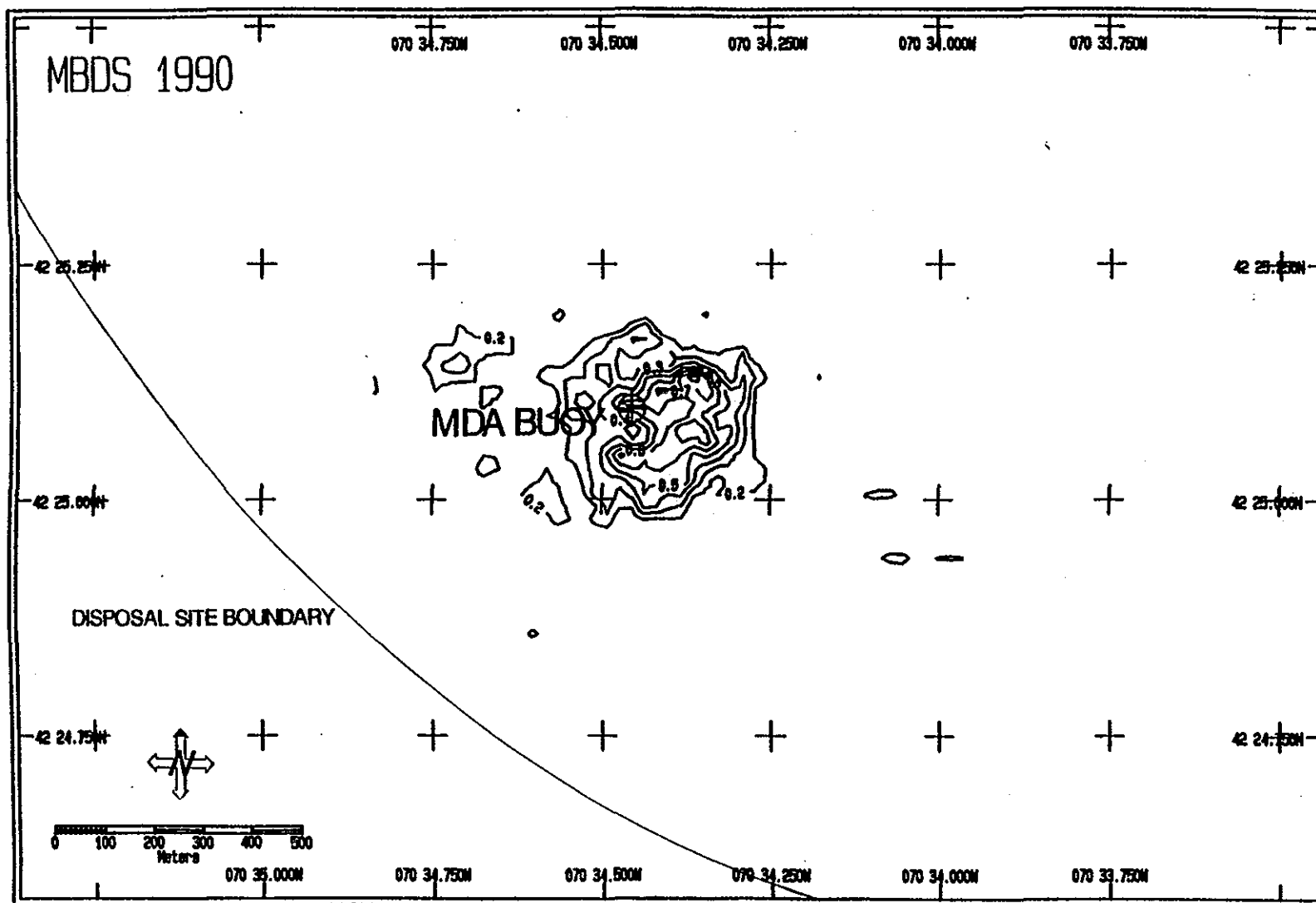
Figure 3-3. Depth difference (in meters) contour map based on comparison of the November 1988 and August 1990 precision bathymetric surveys at the "MDA" buoy
