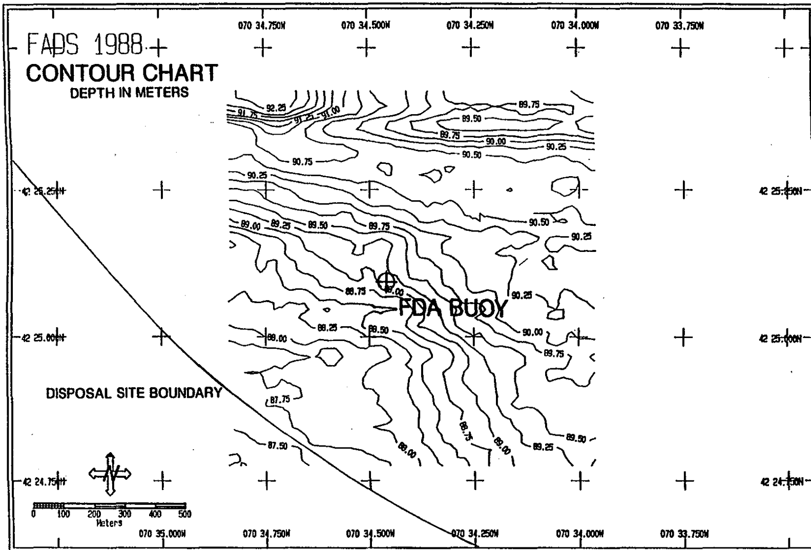
Figure 3-2. Contoured bathymetric chart (in meters) of the area surrounding the "FDA" buoy at MBDS, November 1988
