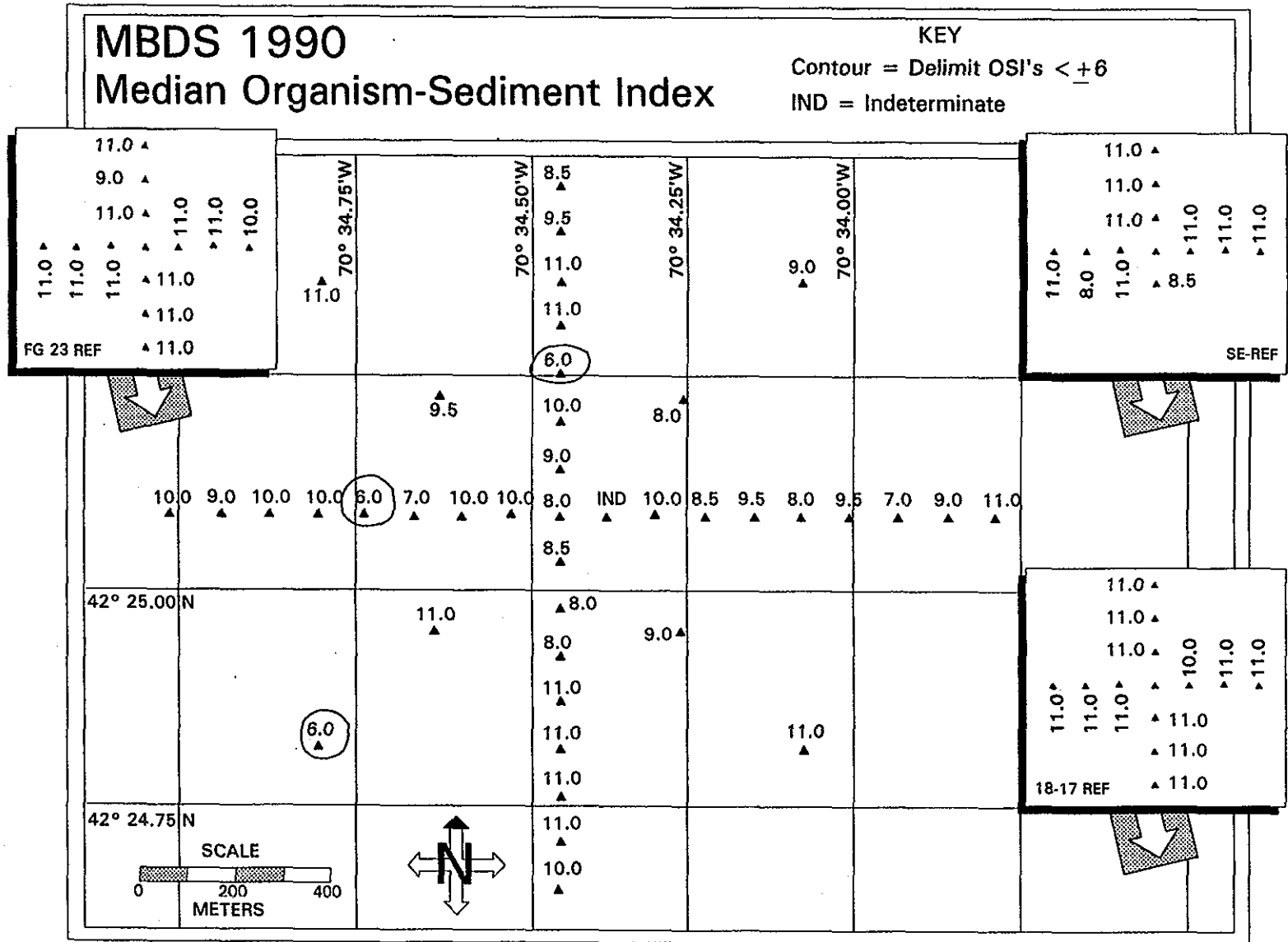
Figure 3-14. The median Organism-Sediment Index (OSI) values for MBDS, August 1990
