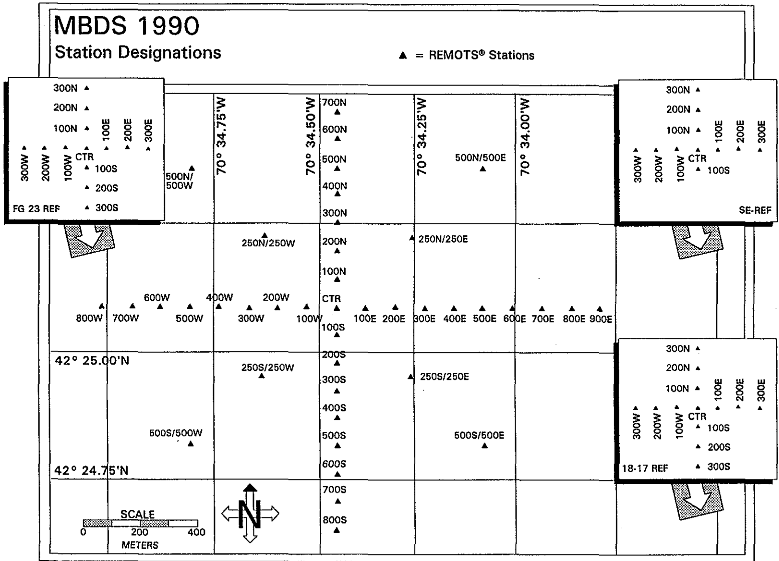
Figure 2-2. REMOTS® station locations at MBDS, August 1990
