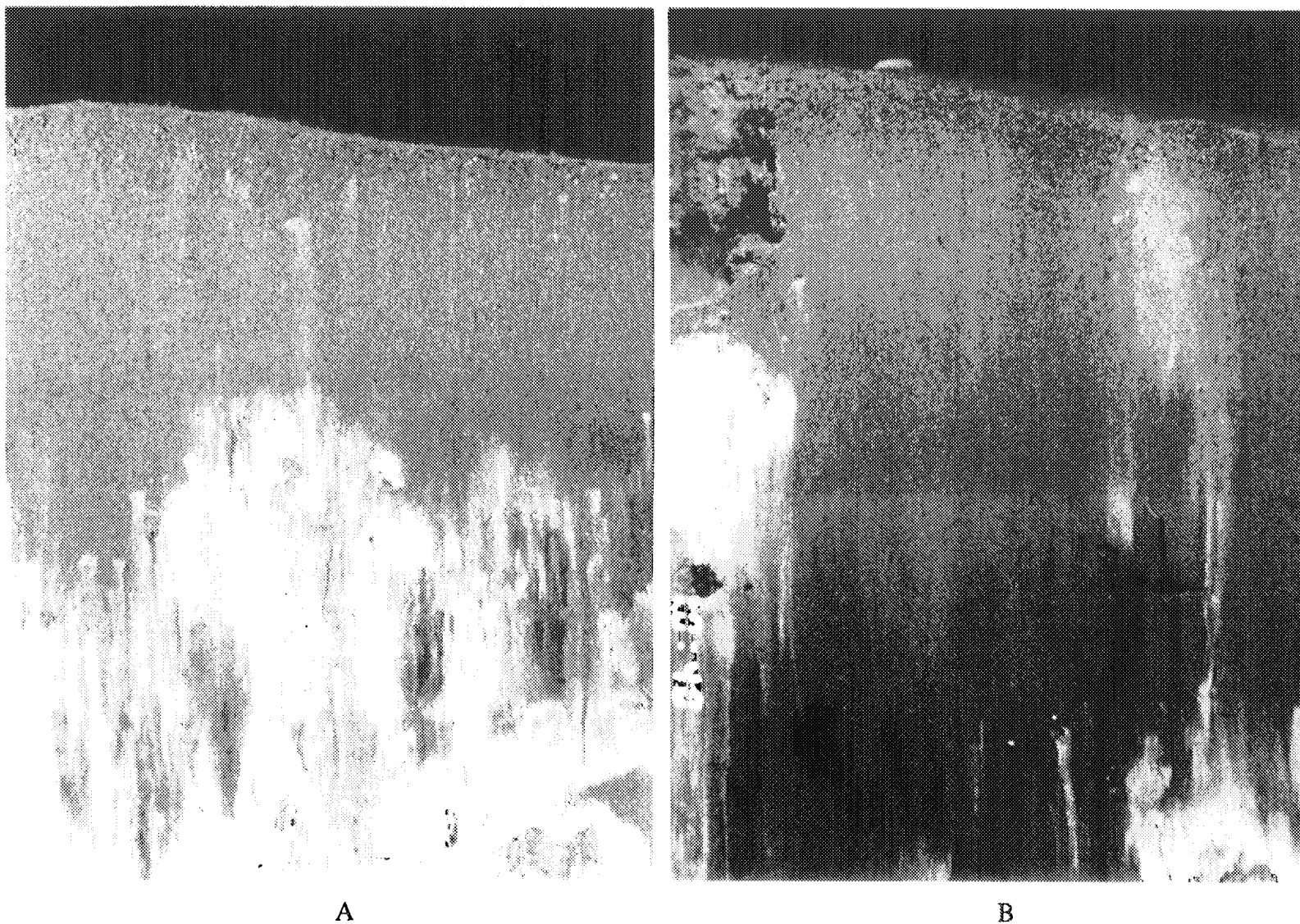
Figure 3-9. REMOTS® photographs from stations 300W (A) and 800W (B) showing a "chaotic" mixture of silts, fine sands, and sands intermixed with clay in the recently disposed dredged material (magnification 1×)
