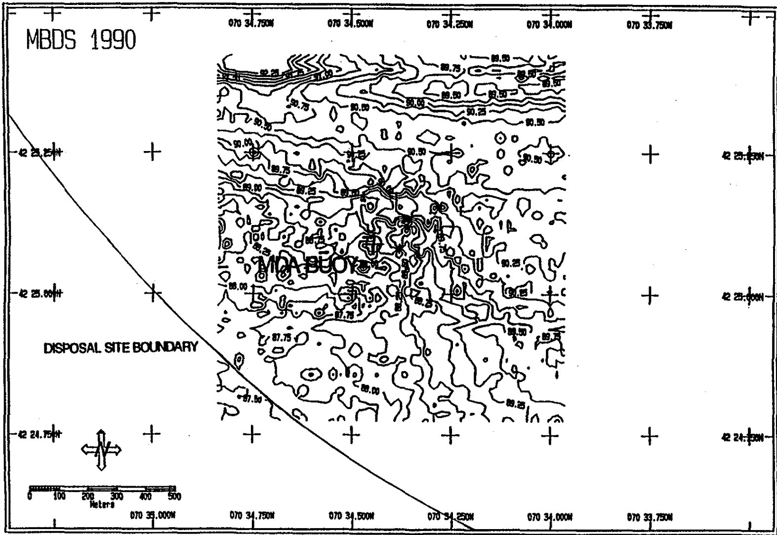
Figure 3-1. Contoured bathymetric chart (in meters) of the area surrounding the "MDA" buoy (former "FDA" buoy) at MBDS, August 1990
