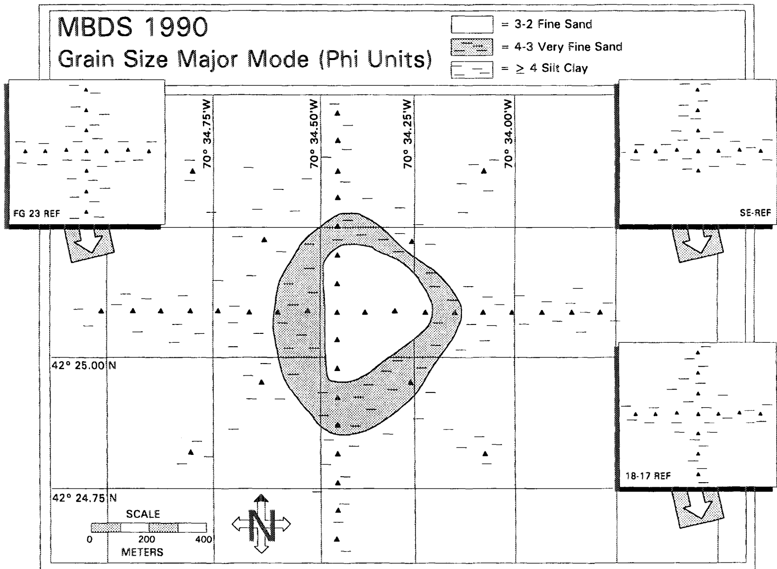
Figure 3-4. Map of sediment grain size major mode for MBDS, August 1990
