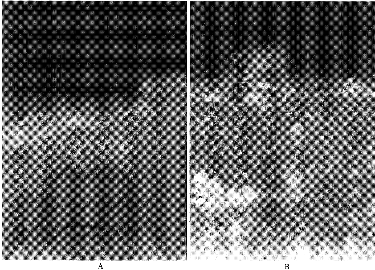
Figure 3-6. REMOTS ® photographs from station 300E (A) and the disposal site center (B); anomalous grain sizes indicated the presence of dredged sediments (magnification 1×)
