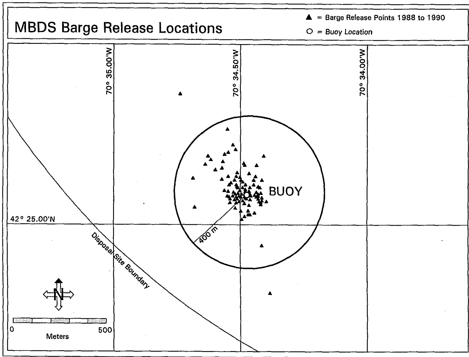
Figure 4-1. A plot of the barge release points for 1988-1990. The plot indicates that the majority of barges released dredged sediments within 400 m of the buoy location.
