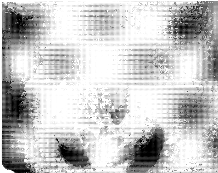
Figure 3-54. A lobster out of its burrow at the disposal mound.
