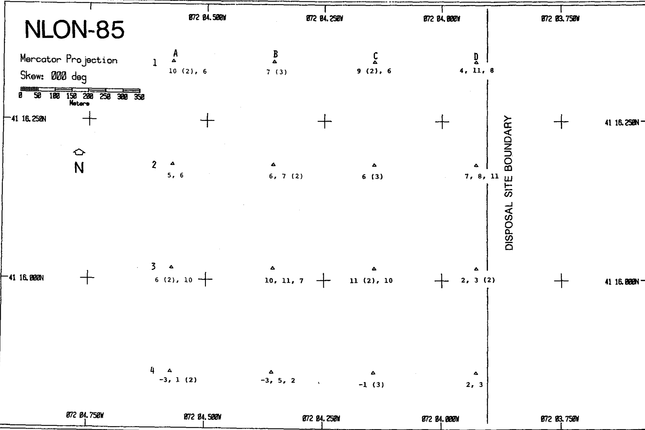
Figure 3-30. The distribution of OSI values at the NLON-85 survey area, November 1985.
