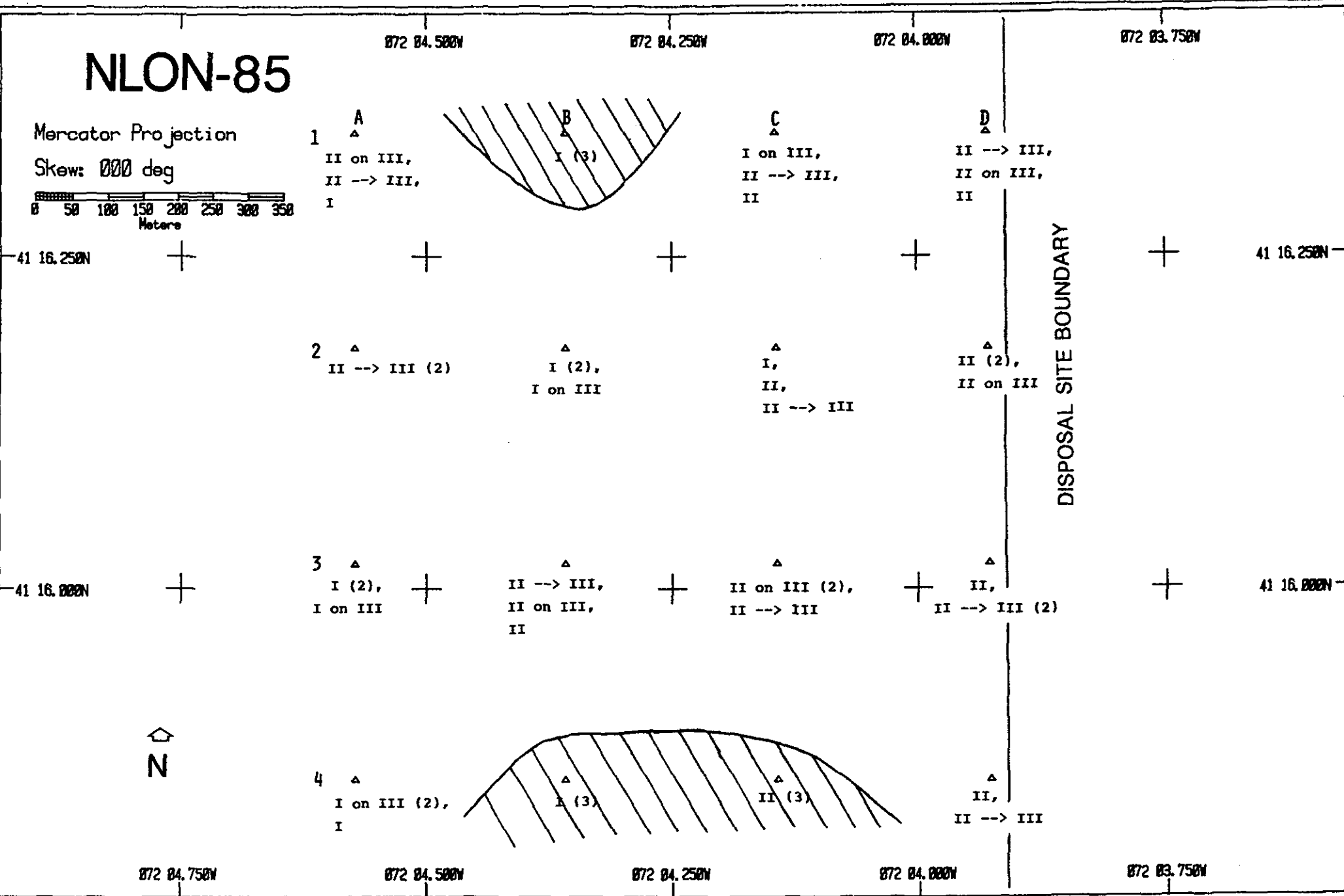
Figure 3-28. The distribution of infaunal successional seres at the NLON-85 survey area, November 1985. The hatched areas lacked evidence of high-order successional infauna (Stage III).
