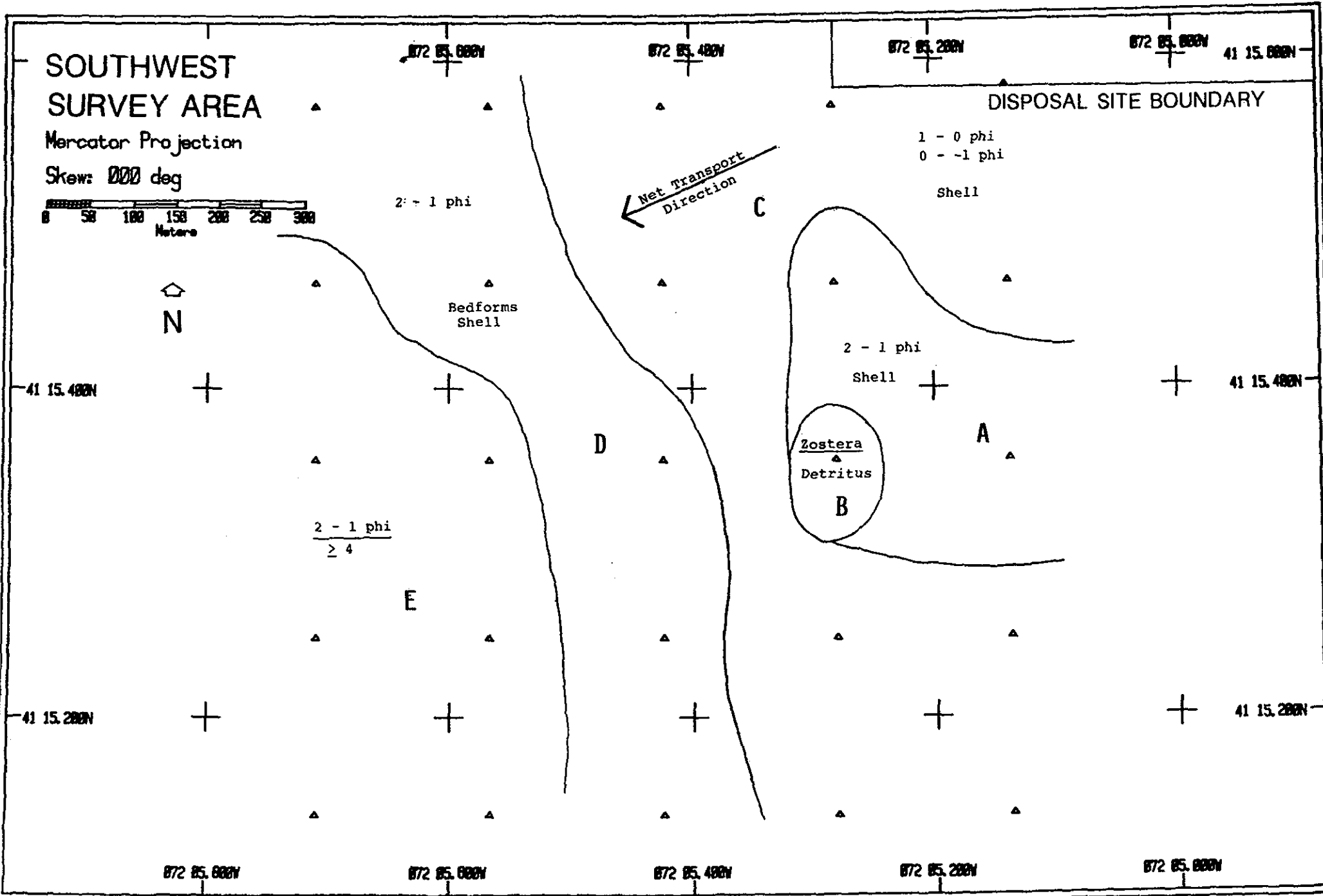
Figure 3-20. The distribution of grain-size major mode at the Southwest survey area, August 1985. Five sedimentary facies, A through E, were identified (see text for further discussion).
