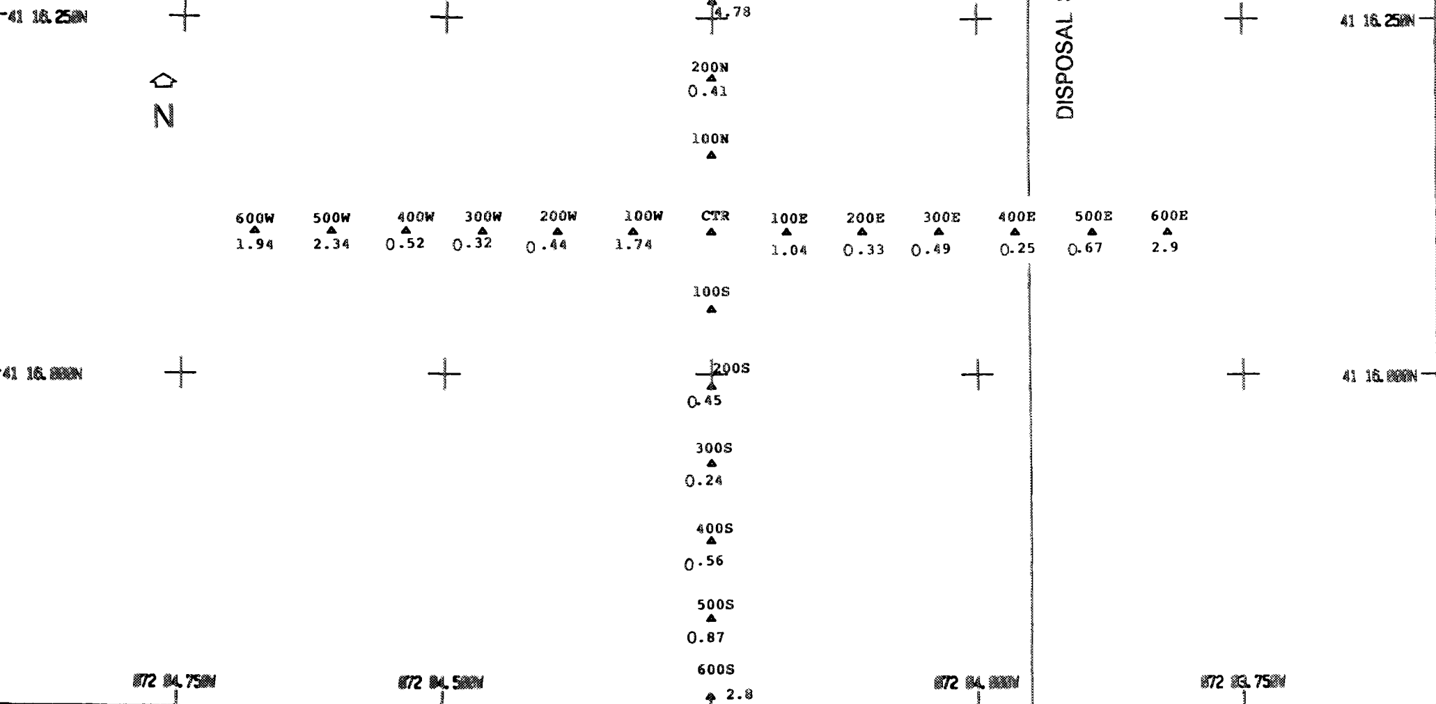
Figure 3-34. The distribution of mean apparent RPD depths at the NLON-85 survey area, January 1986. RPD depths could not be measured at unlabeled stations due to overpenetration of the camera prism.
