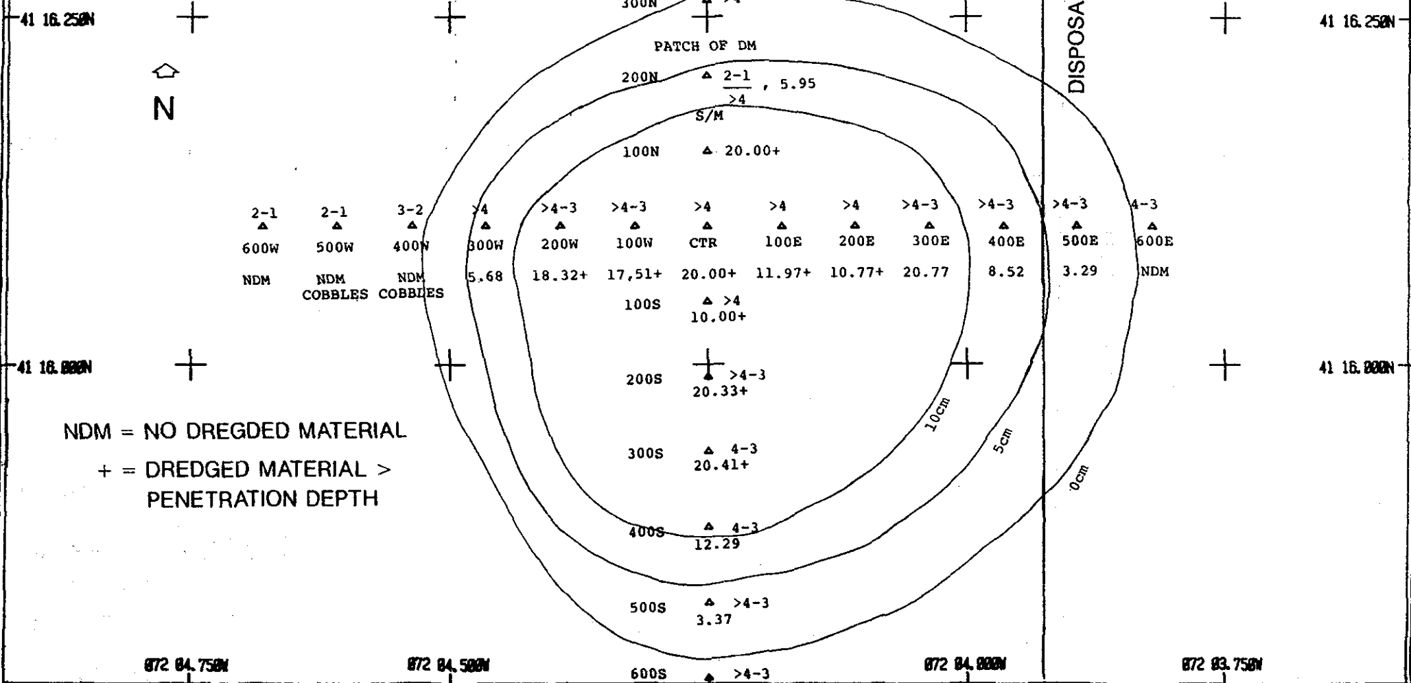
Figure 3-31. The distribution and thickness of dredged material at the NLON-85 survey area, January 1986. Grain size (phi units) is reported above the station label. The thickness values below the station label are in cm.
