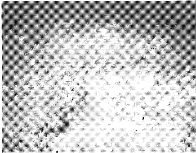
Figure 3-58. A crustacean foraging excavation.
