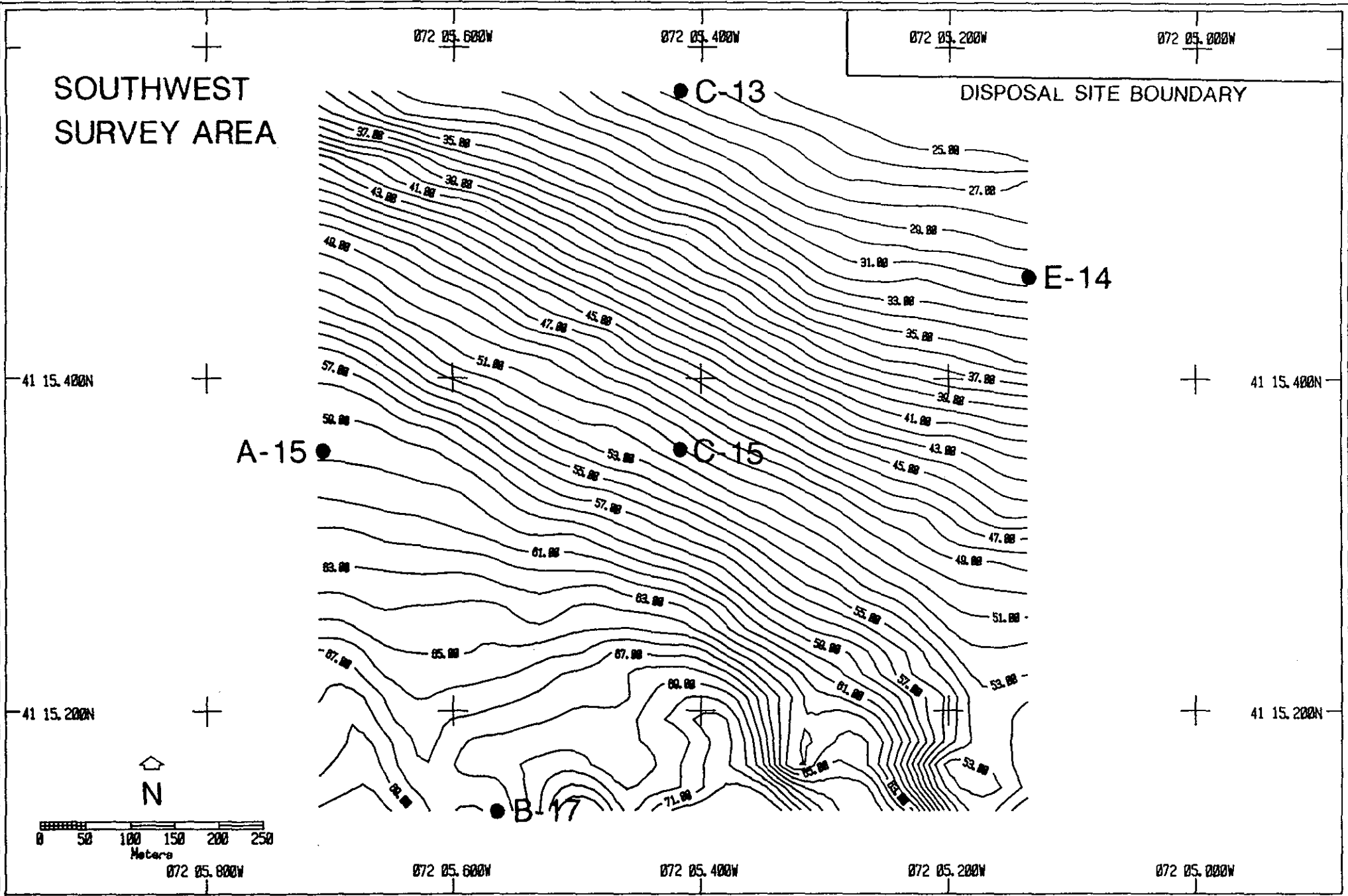
Figure 3-2. Contoured bathymetric chart of an area immediately southwest of the New London Disposal Site, July 1985. Depths are in meters. Sediment sampling stations are indicated.
