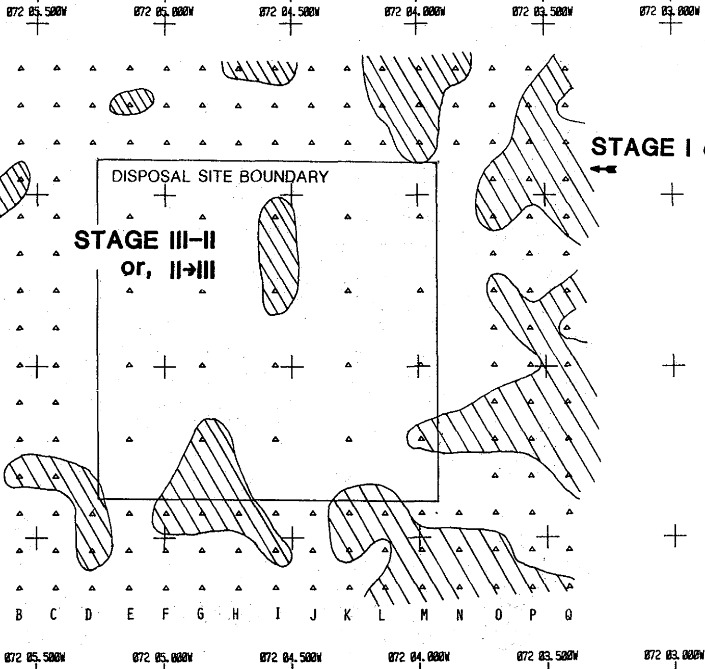
Figure 3-15. The distribution of infaunal successional stages at the New London Disposal Site, July 1985. The hatched areas were characterized by Stage I or II seres. The remainder of the area exhibited Stage III-II or II->III assemblages.
