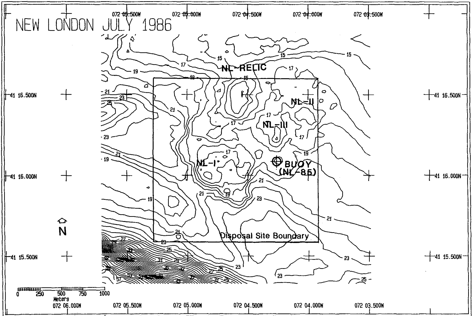
Figure 3-6. Contoured bathymetric chart of the New London Disposal Site, July 1986. Depths in meters.
