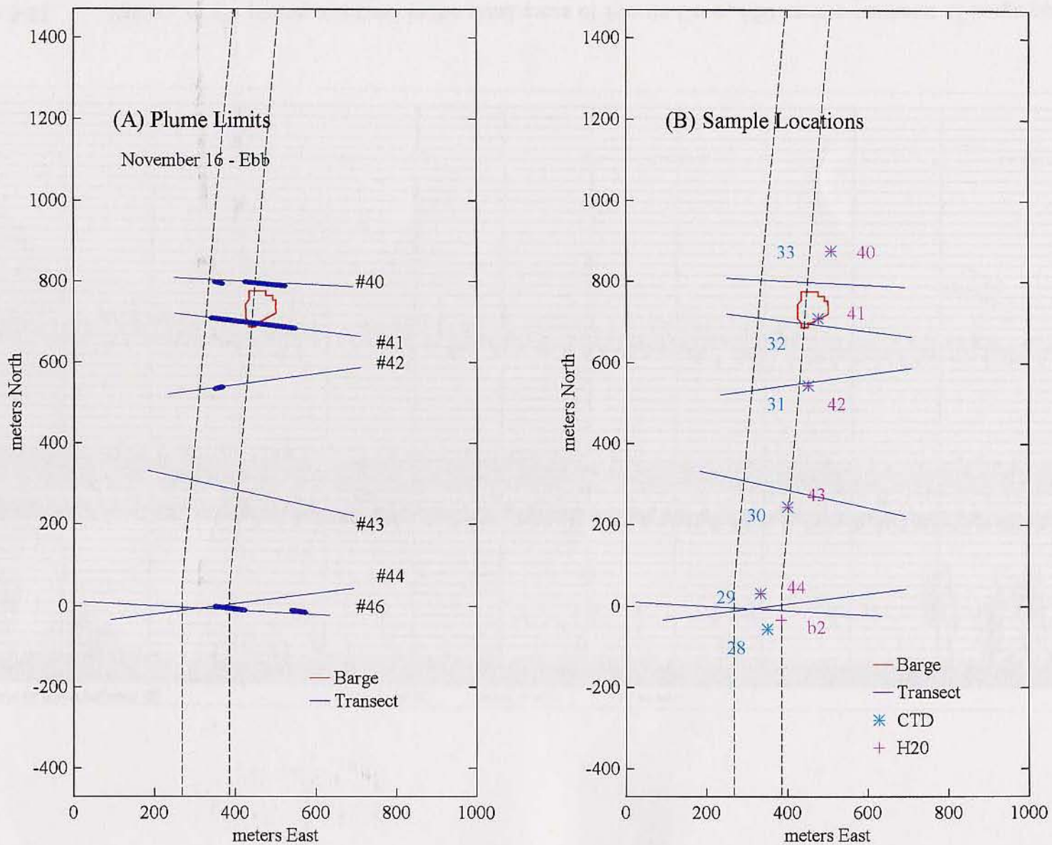
Figure 3-22. (A) November 16, 1993 barge position and transect locations with the occurrence of the plume delineated on each transect; (B) barge position and transects with the location of water samples
