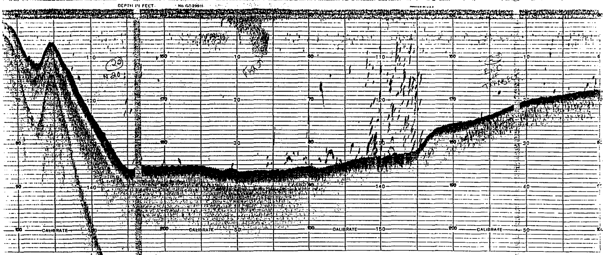
Figure 3-7. Echo sounder trace of Transect I showing patches of plume 250 meters downstream of the barge on October 25. The profile runs east to west.
