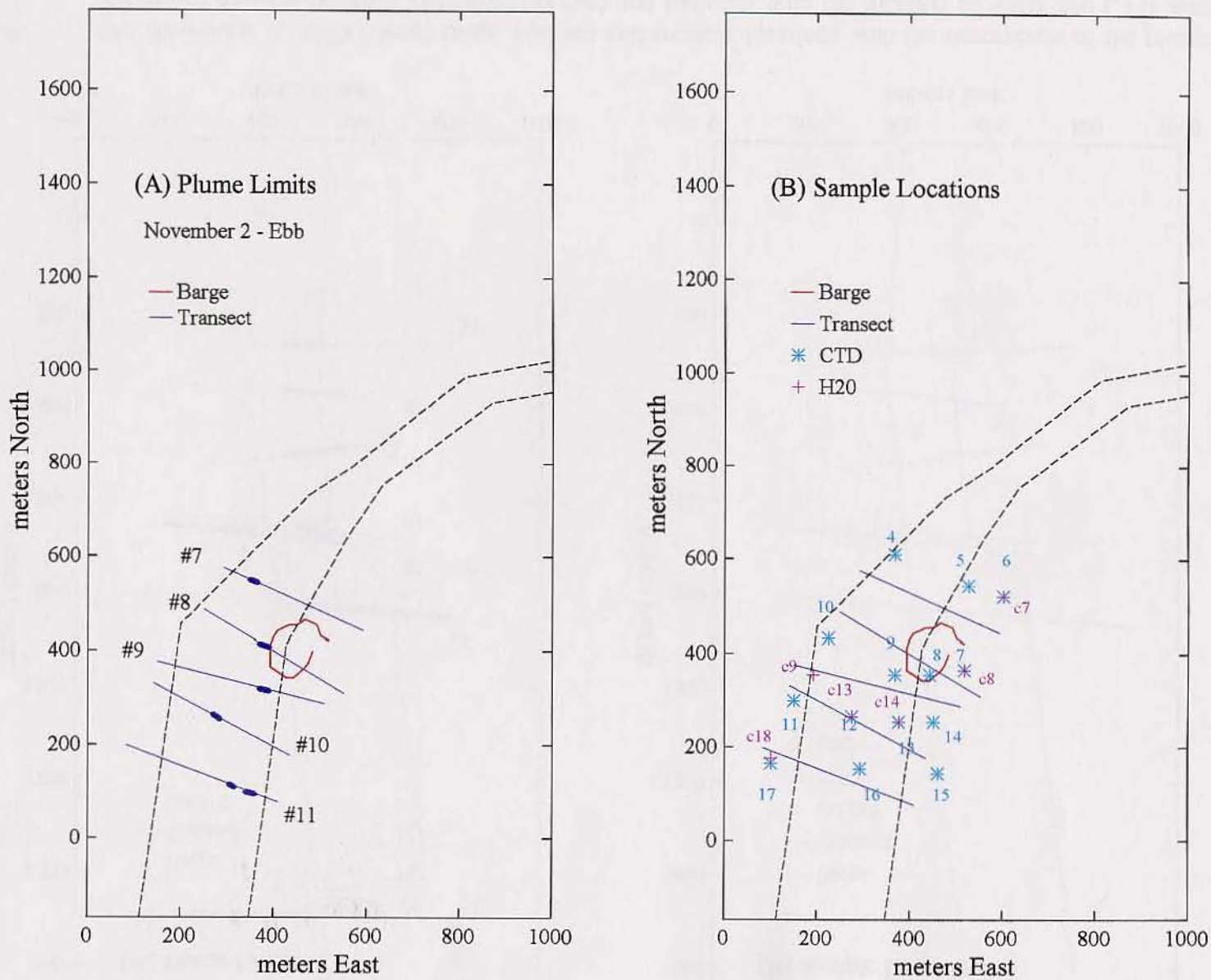
Figure 3-10. (A) November 2, 1993 (ebb) barge position and transect locations with the occurrence of the plume delineated on each transect; (B) barge position and transects with the location of water and CTD samples
