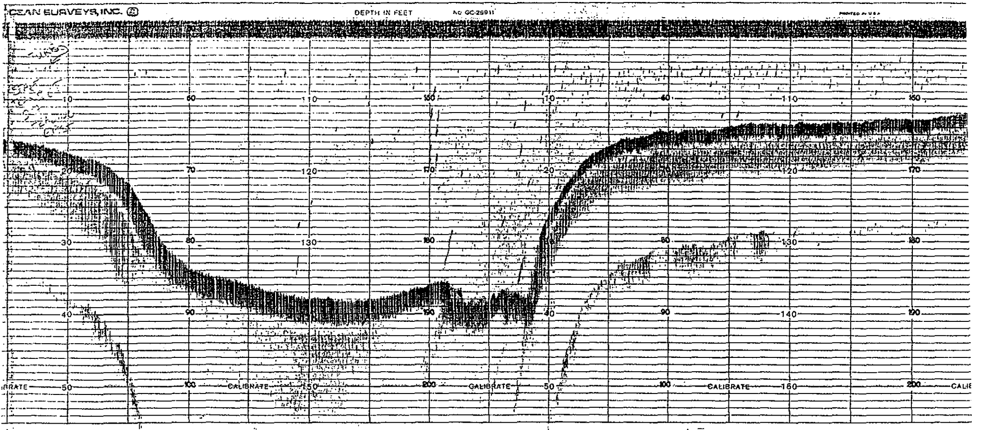
Figure 3-16. Traces of the plume from the echo sounder records of Transect #27, advected 525 meters downcurrent along the eastern boundary of the channel, November 11. Profile runs west to east.
