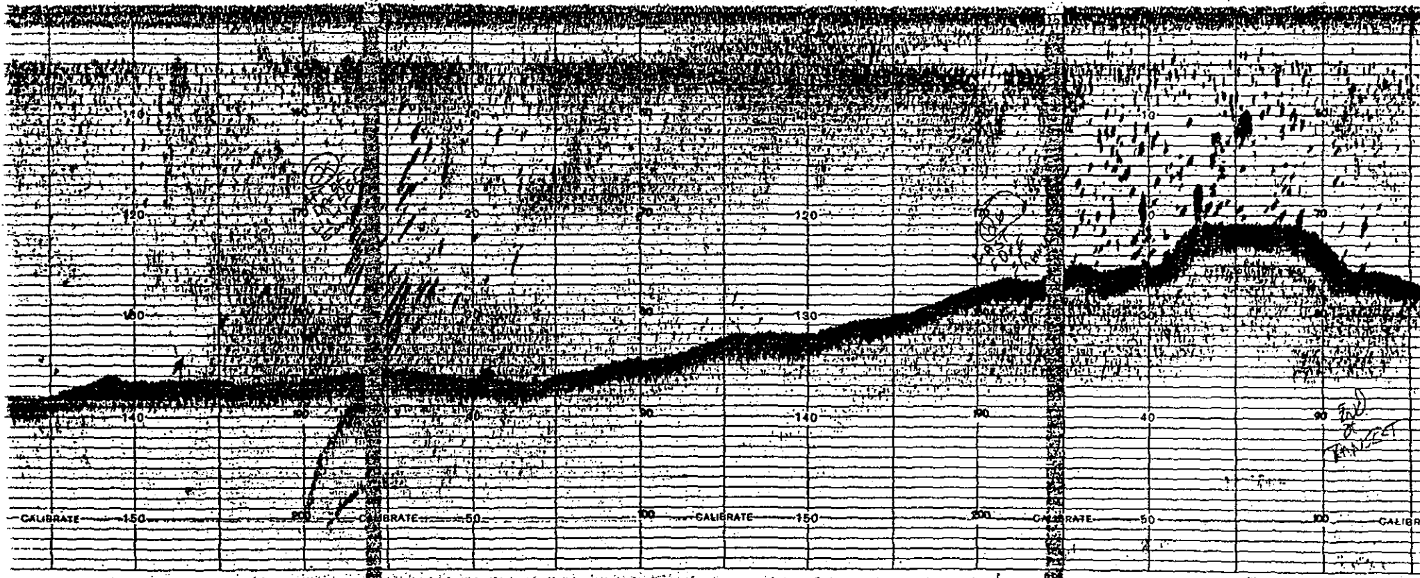
End segment of Transect J acoustic profile surveyed on 25 October 1993; profile runs west to east
