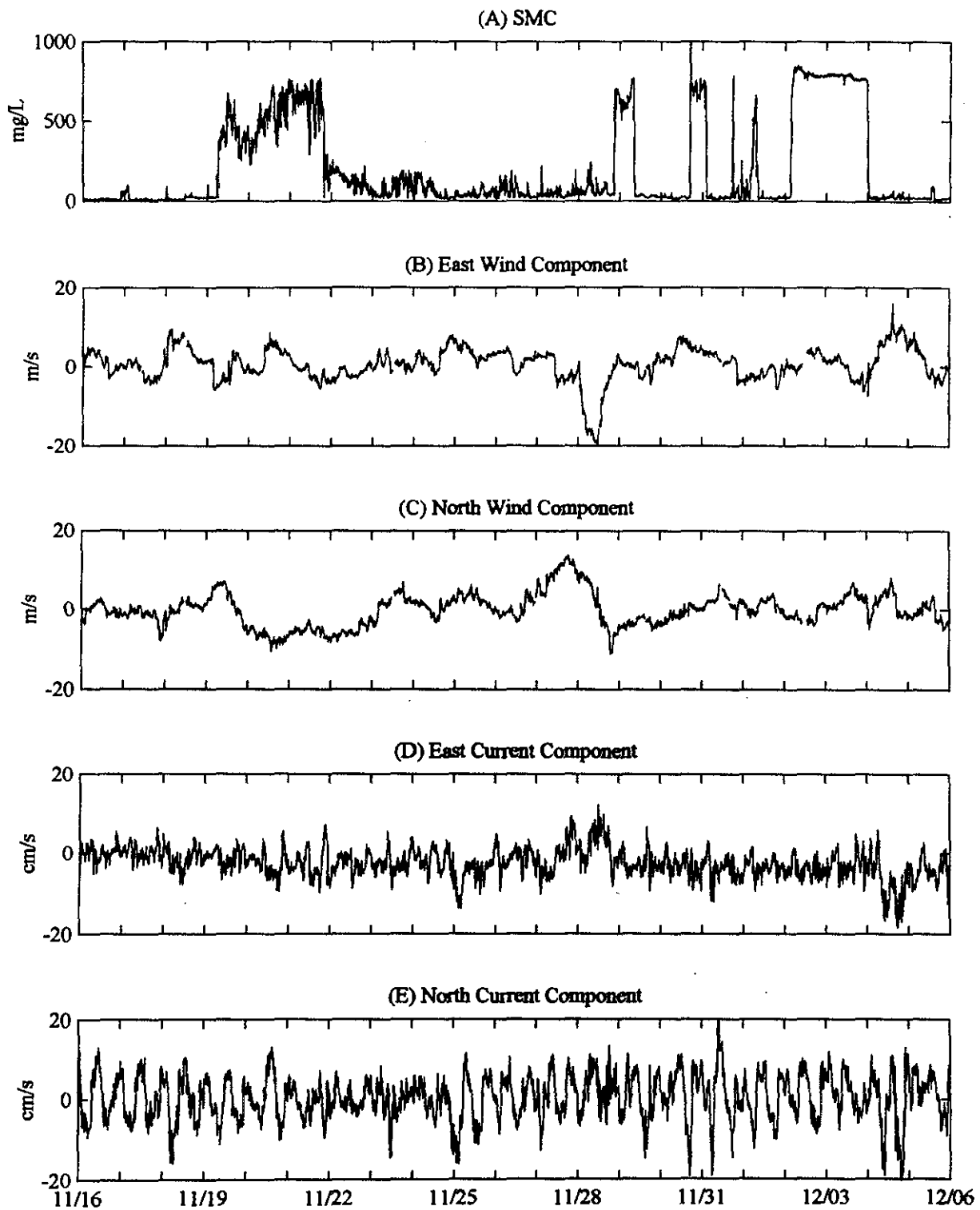
Figure 3-32. Enlargement of the period during which the largest SMC perturbations were observed, November 16 to December 6, 1993. Concentration data are compared with wind and current data.
