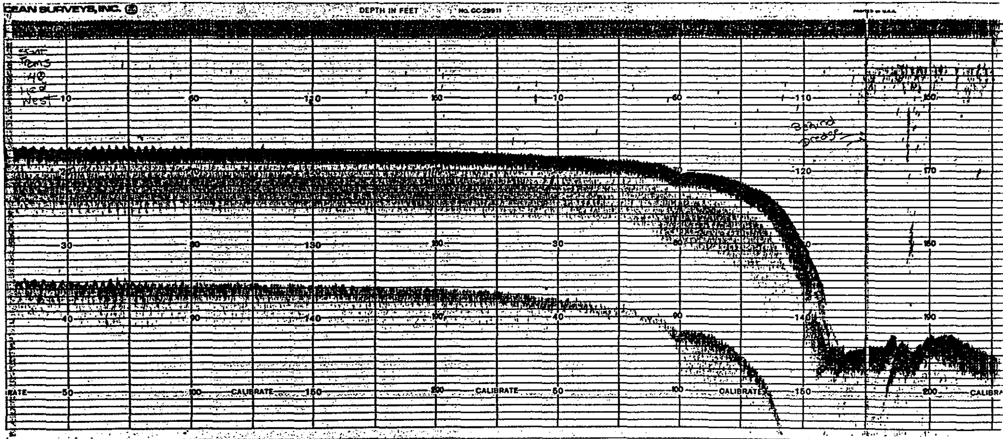
Beginning segment of Transect #42 acoustic survey of 16 November 1993; profile runs east to west
