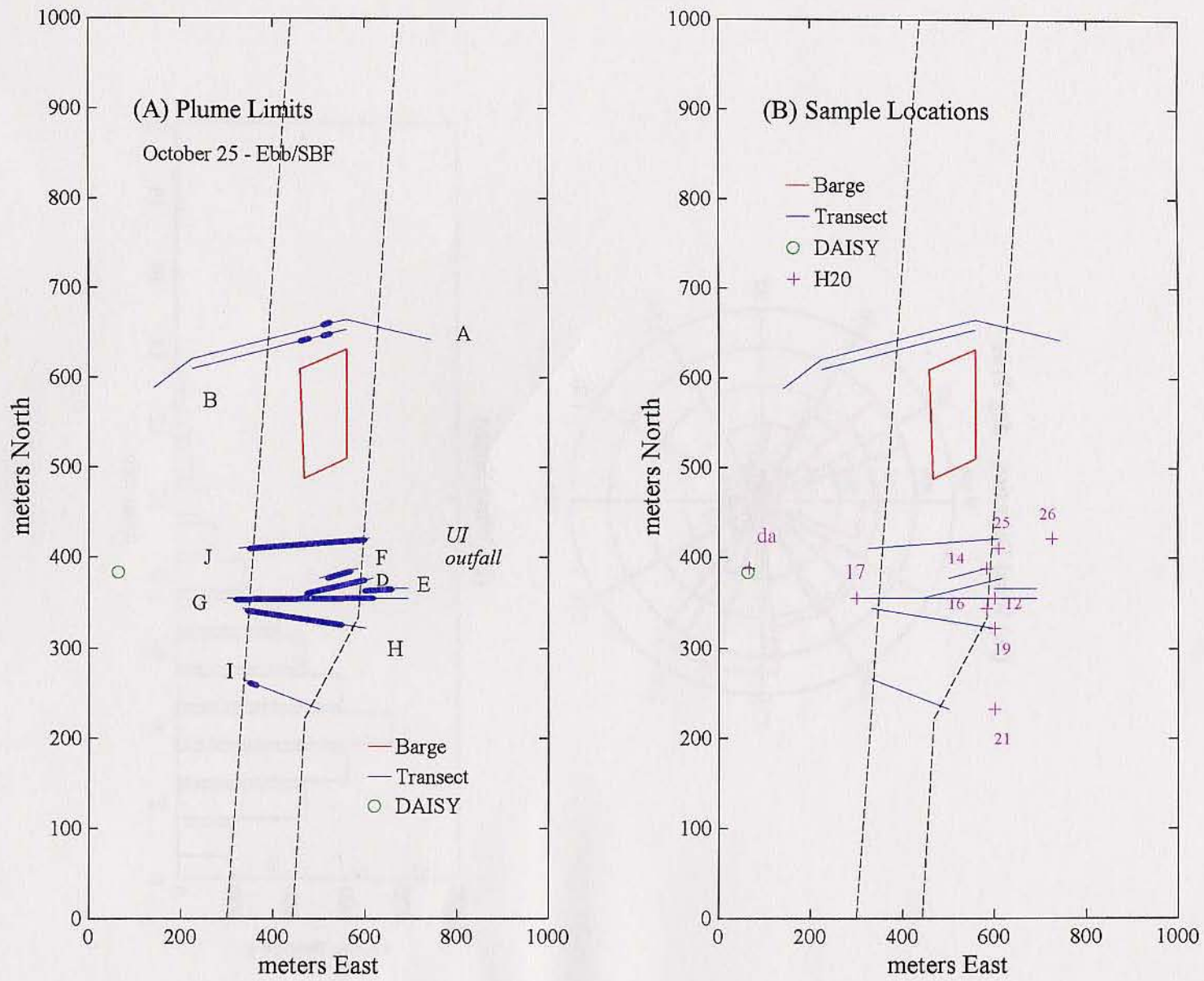
Figure 3-6. (A) October 25, 1993 barge position and transect locations with the occurrence of the plume delineated on each transect; (B) barge position and transects with the location of water samples
