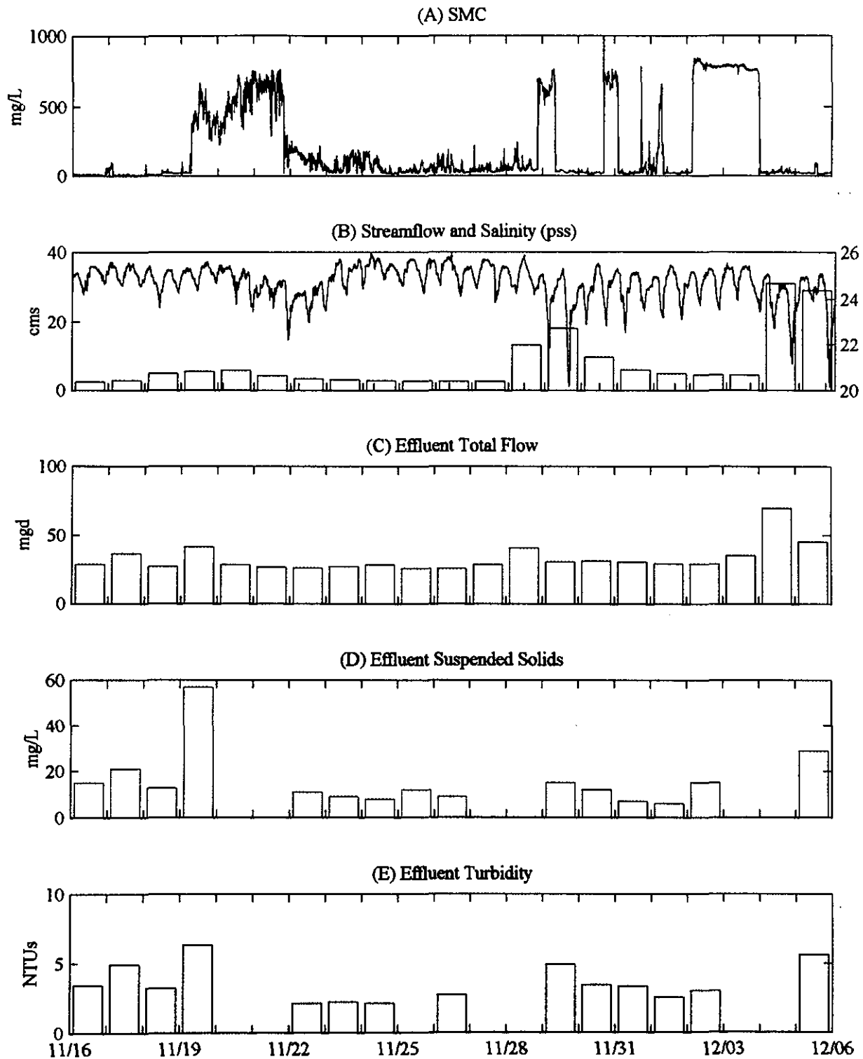
Figure 3-33. The suspended material concentration data compared with stream flow and effluent data obtained from the East Haven Pollution Abatement Facility for the period November 16 to December 6, 1993
