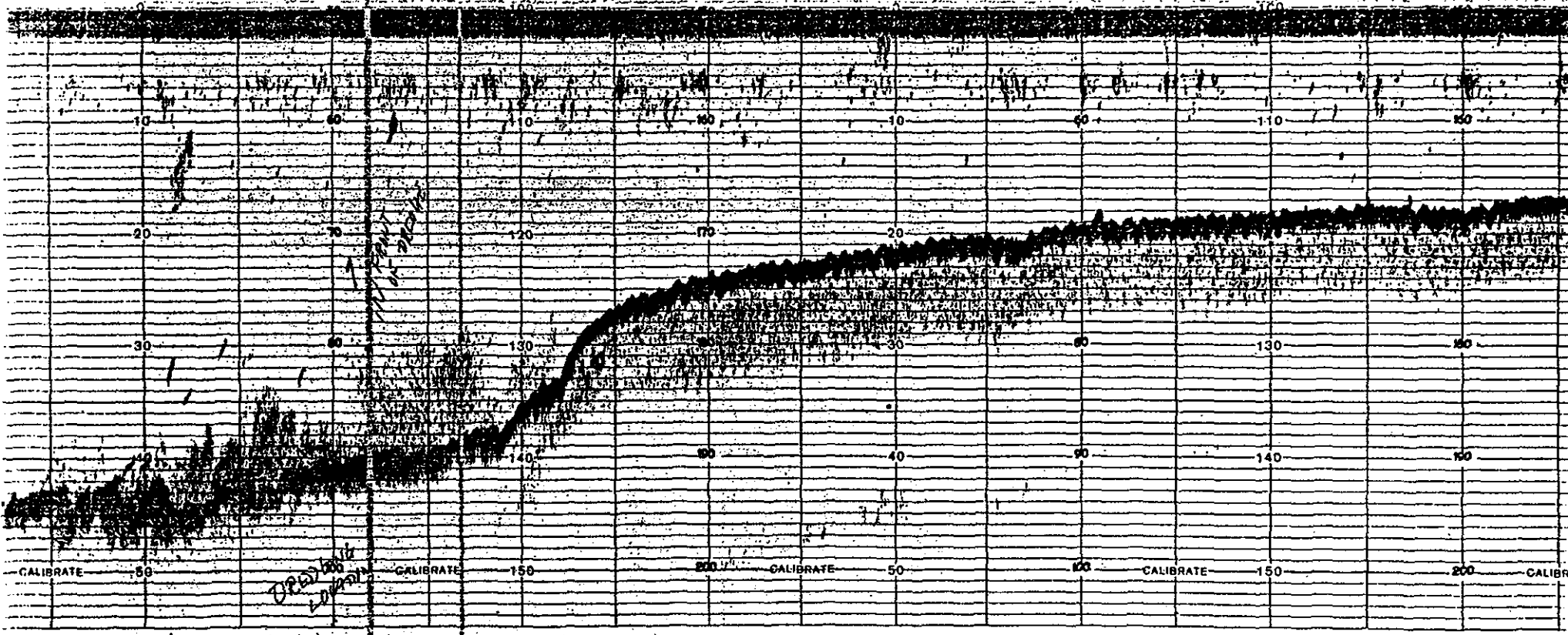
End segment of Transect #13 acoustic survey of 3 November 1993; profile runs east to west
