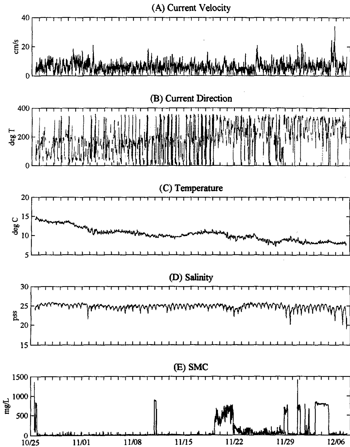
Figure 3-26. Time series plots for the complete DAISY deployment period, October 25 to December 7, 1993
