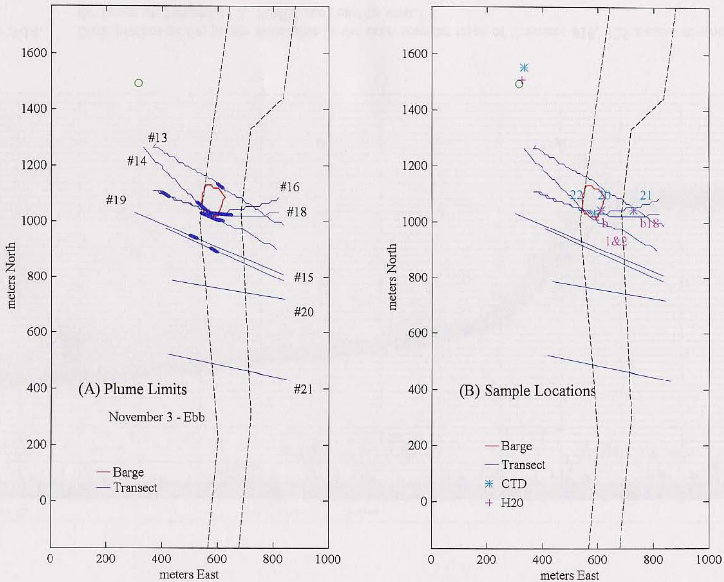
Figure 3-13. (A) November 3, 1993 barge position and transect locations with the occurrence of the plume delineated on each transect; (B) barge position and transects with the location of water and CTD samples
