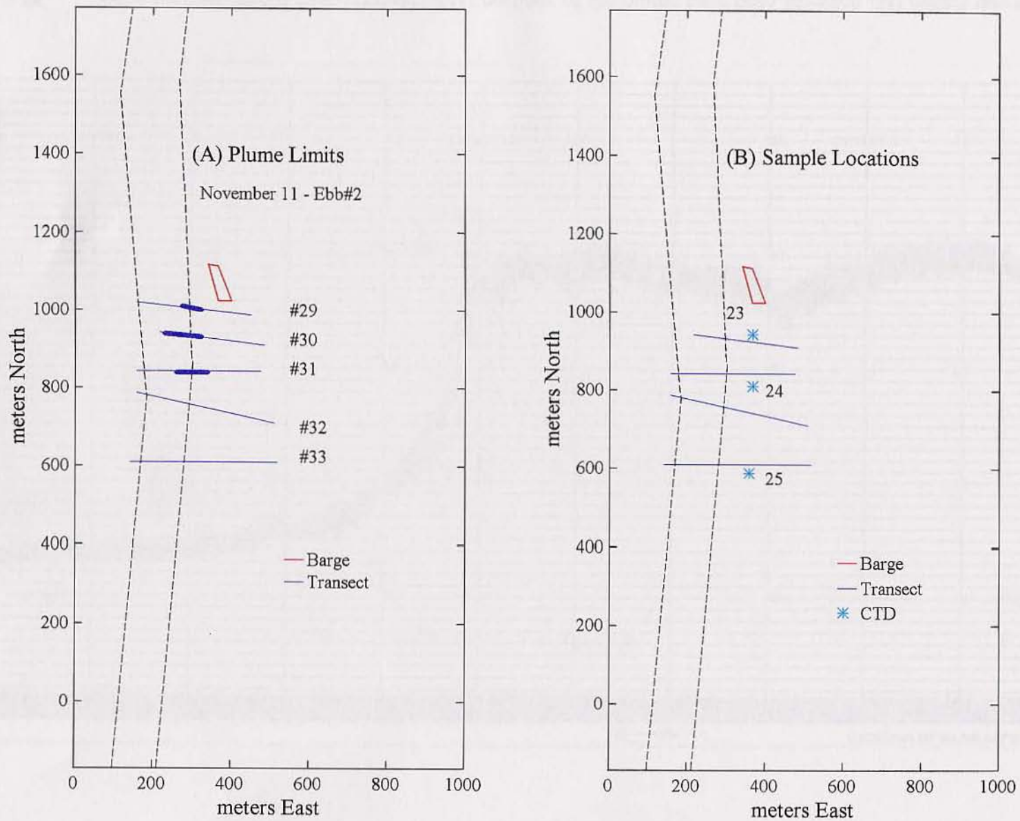
Figure 3-17. (A) November 11, 1993 (second ebb survey) barge position and transect locations with the occurrence of the plume delineated on each transect; (B) barge position and transects with the location of water samples
