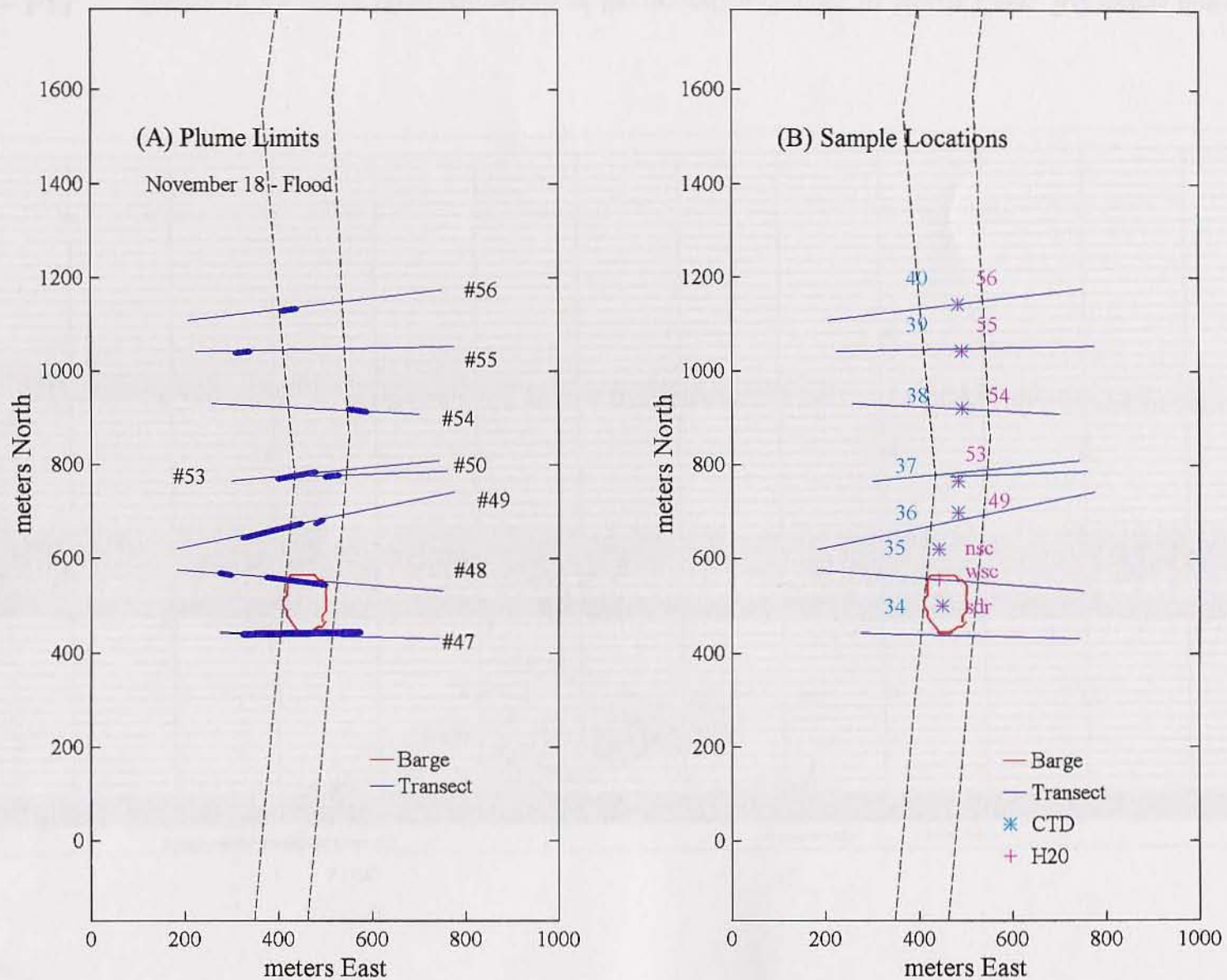
Figure 3-24. (A) November 18, 1993 barge position and transect locations with the occurrence of the plume delineated on each transect; (B) barge position and transects with the location of water samples
