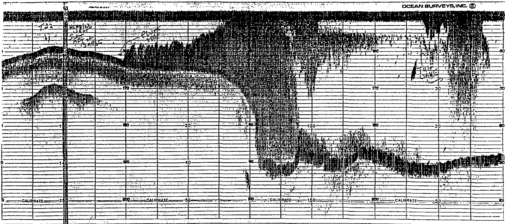
Beginning segment of Transect #22 acoustic survey of 11 November 1993; profile runs east to west
