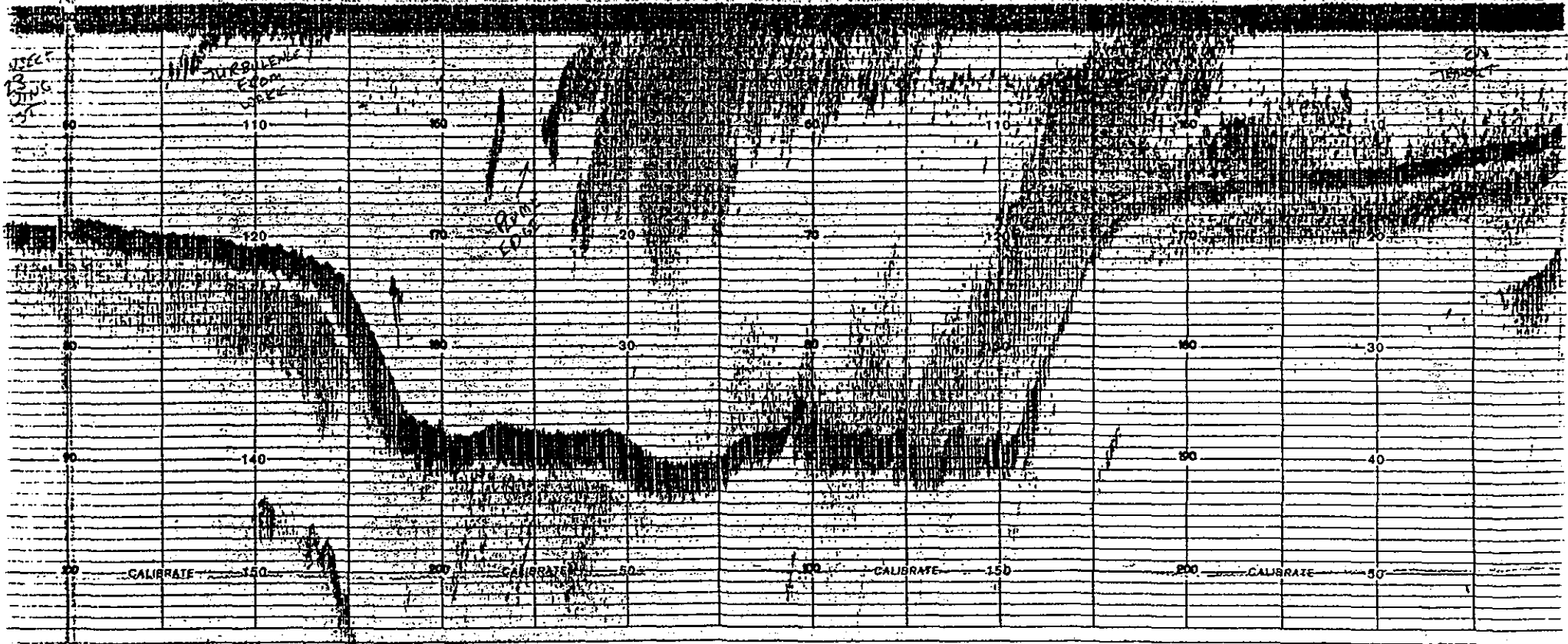
Transect #23 acoustic survey of 11 November 1993; profile runs west to east
