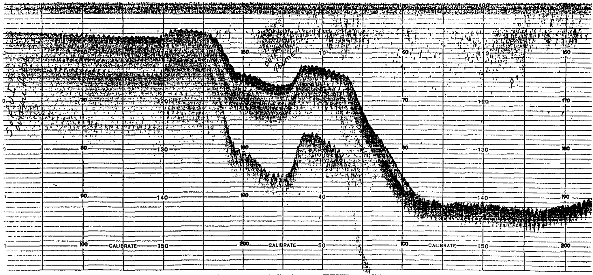
Beginning segment of Transect #3 acoustic survey of 2 November 1993; profile runs east to west
