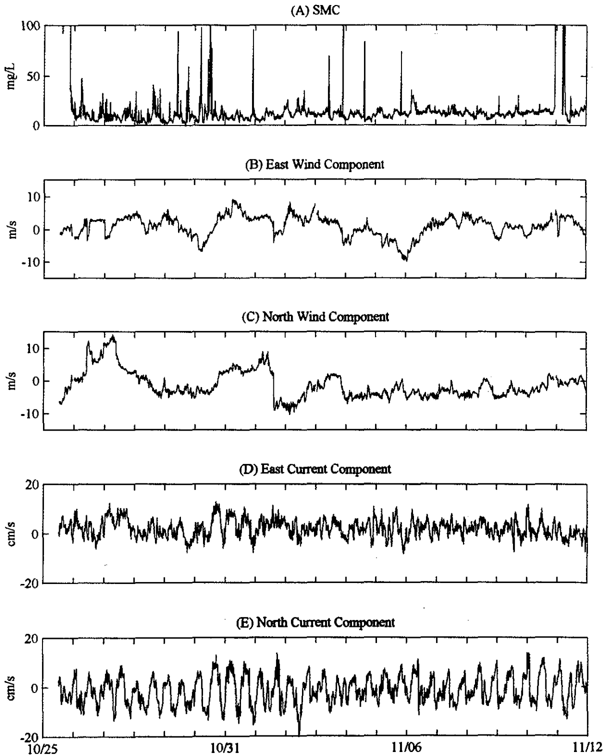
Figure 3-30. The suspended material concentration data compared with wind and current data for the first half of the deployment, October 25 to November 11, 1993
