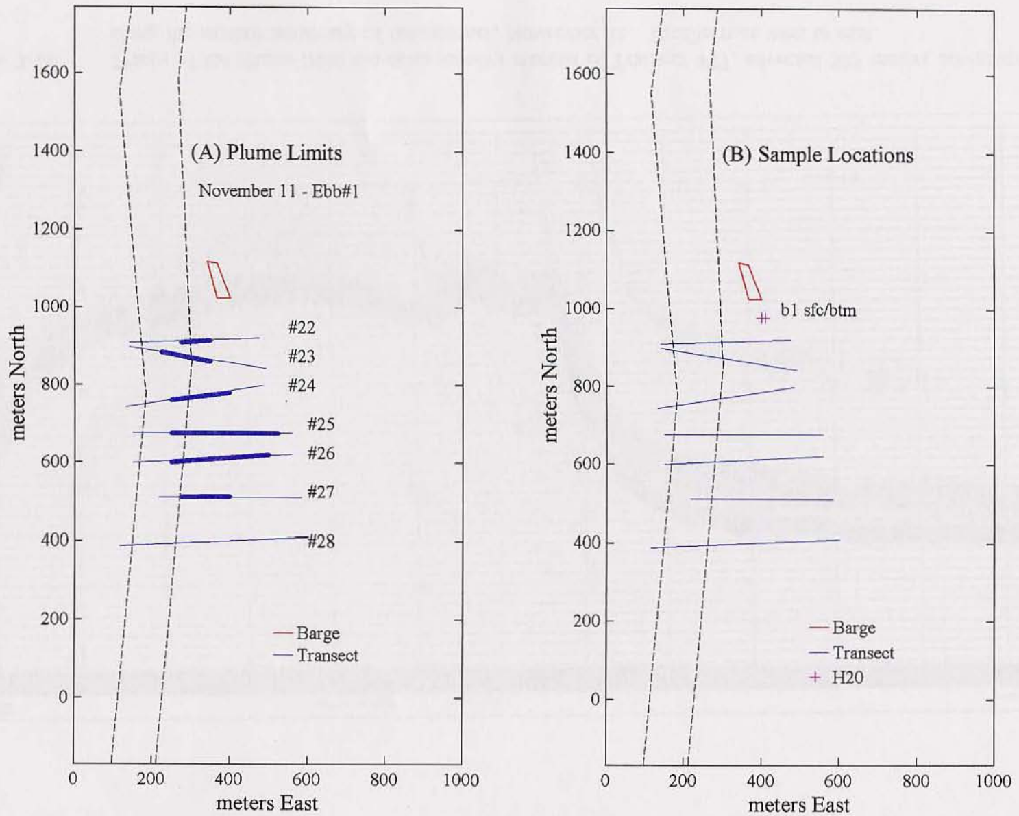
Figure 3-15. (A) November 11, 1993 (first ebb survey) barge position and transect locations with the occurrence of the plume delineated on each transect; (B) barge position and transects with the location of water samples
