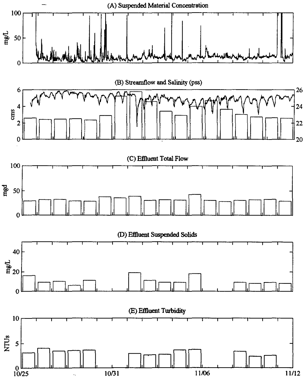
Figure 3-31. The suspended material concentration data compared with stream flow and effluent from the East Haven Pollution Abatement Facility for the first half of the deployment, October 25 to November 11, 1993
