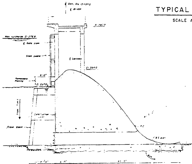
SECTION THRU SPILLWAY & OUTLET WORKS
