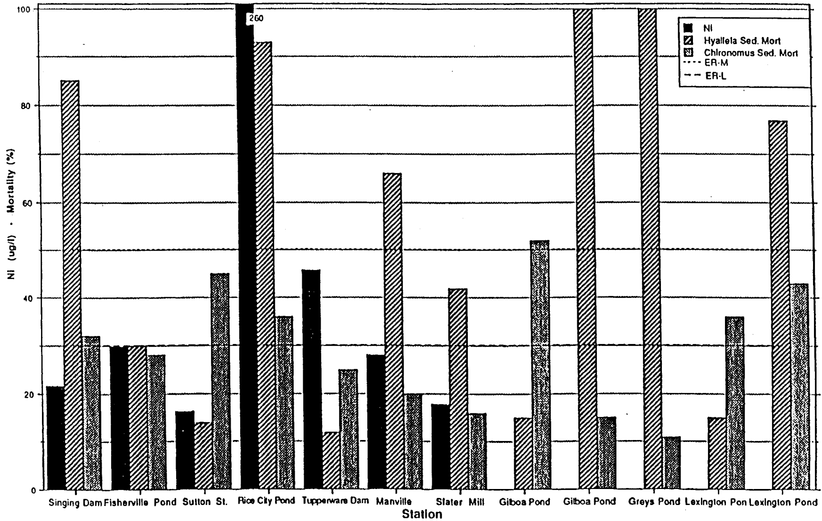
Figure F-5 Nickel in Blackstone River Sediments
