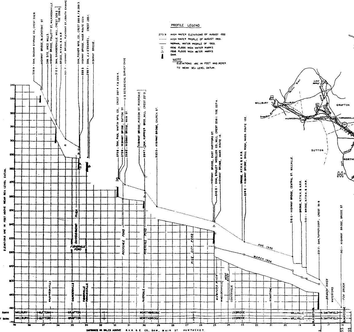
BLACKSTONE RIVER, MI. 16 TO 36. 1955 FLOOD LIMITS SCALE IN MILES DISTANCE IN MILES
