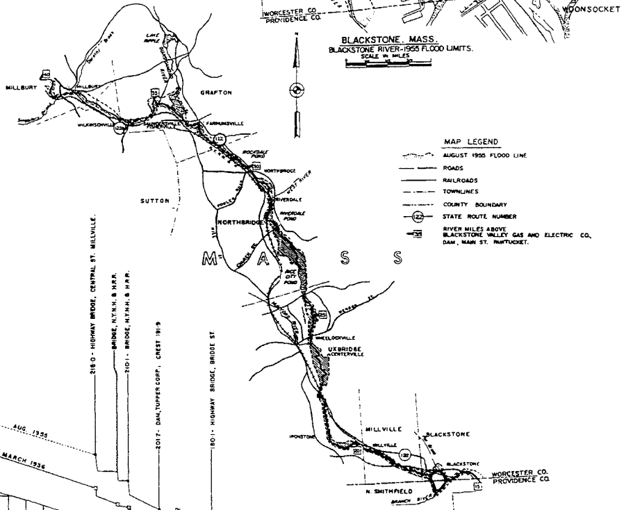
BLACKSTONE RIVER, MI. 16 TO 36. 1955 FLOOD LIMITS SCALE IN MILES DISTANCE IN MILES
