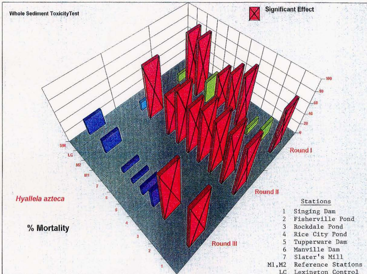
Figure F-9 Results of the Whole Sediment Toxicity Test Hyalallela azteca
