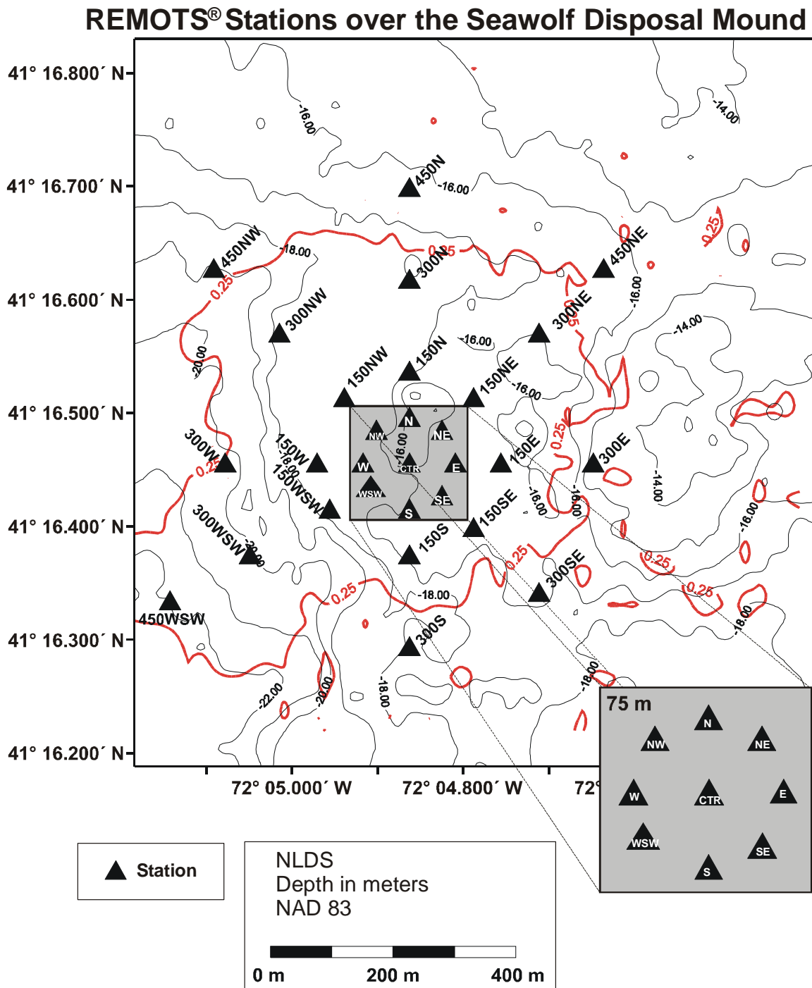
Figure 3-13. Location of Seawolf REMOTS® stations relative to areal extent (0.25 m) of Seawolf dredged material. The Center and 75 m stations are magnified to the right.
