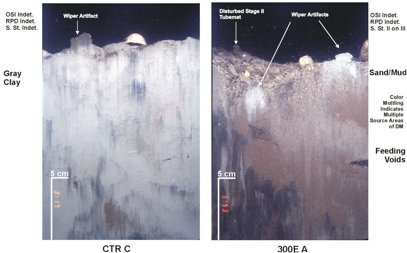
Figure 3- 15. REMOTS ® sediment-profile photographs from 1997 showing variation in CDM over the Seawolf Mound (glacial gray clay at the center station and brown sand and silt at Station 300E A).
