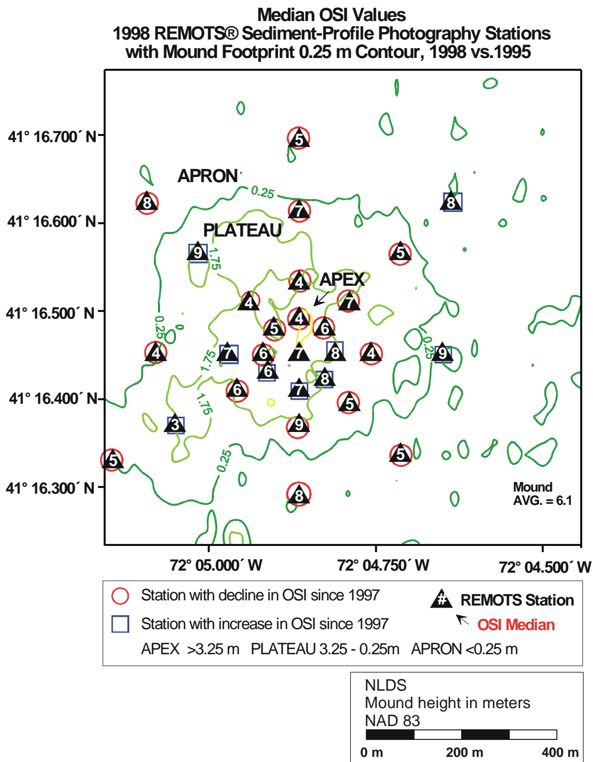
Figure 3-21. Median OSI values over the Seawolf Mound and changes relative to 1997 survey
