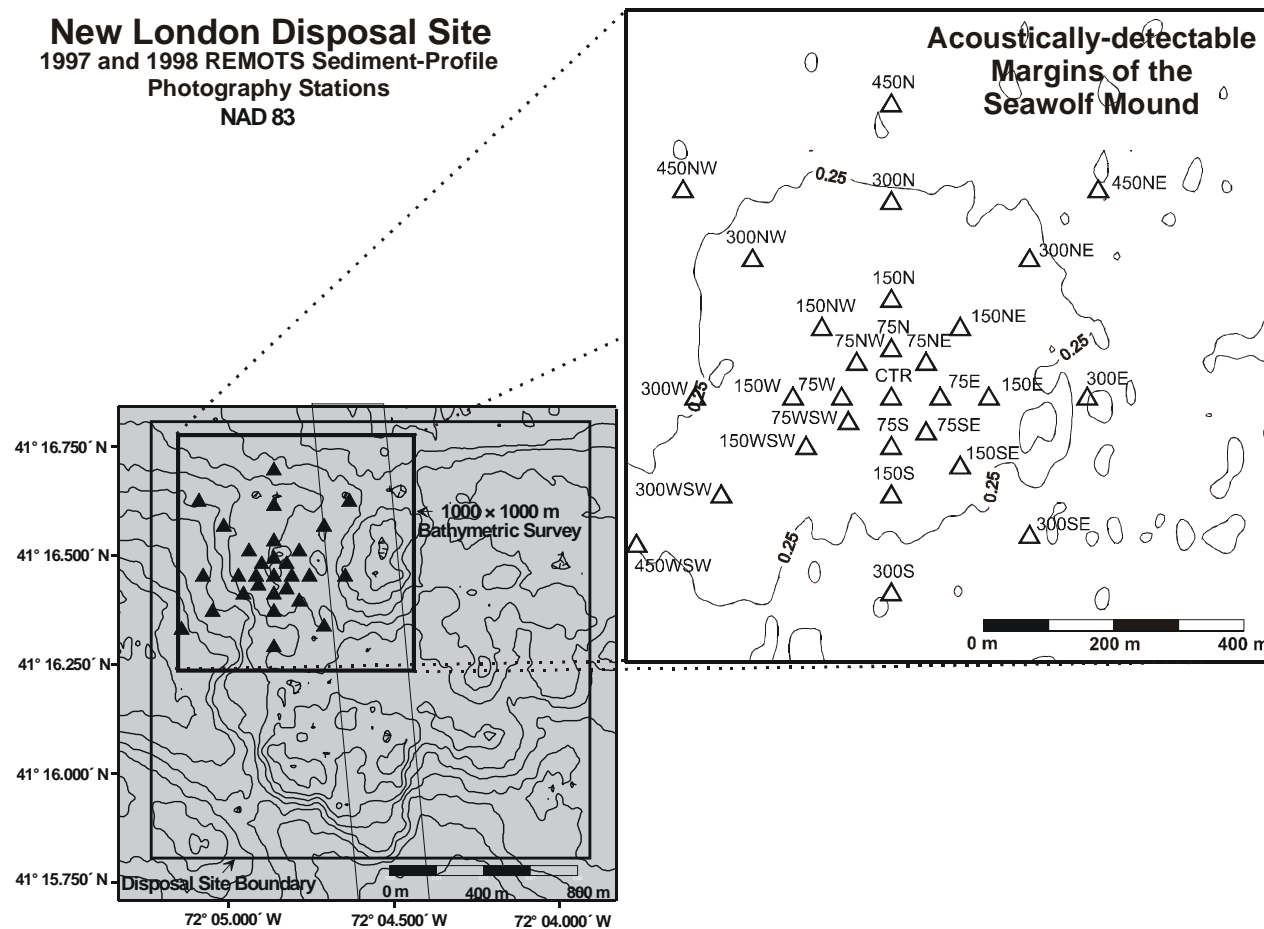
Figure 2-3. Distribution of 1997 and 1998 REMOTS® sediment-profile photography stations (29) over the Seawolf disposal mound, relative to 1000 × 1000 m survey area, disposal site boundary, and US Navy submarine lane.
