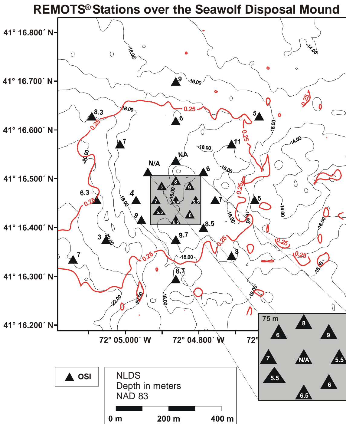
Figure 3- 14. Map of average OSI values at the Seawolf Mound REMOTS® stations in 1997. Note: N/A means that the OSI value was not available or indeterminant.
