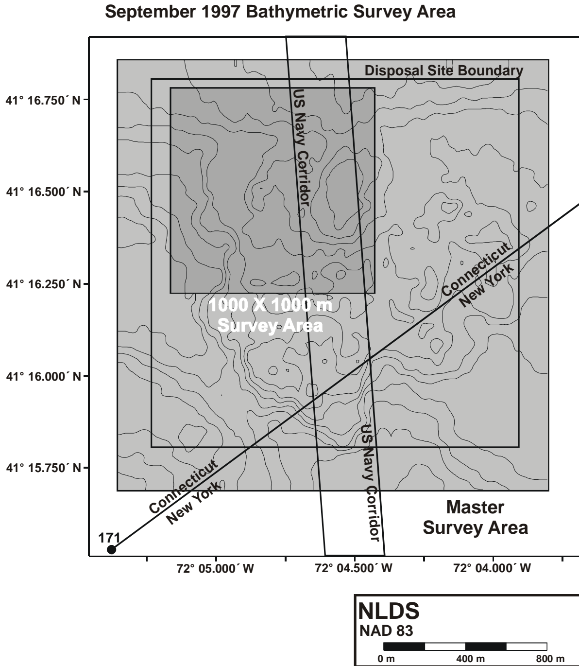
Figure 2-1. Location of the bathymetric survey area over the Seawolf Mound relative to the disposal site boundaries, US Navy submarine lane, and New York-Connecticut State Line.
