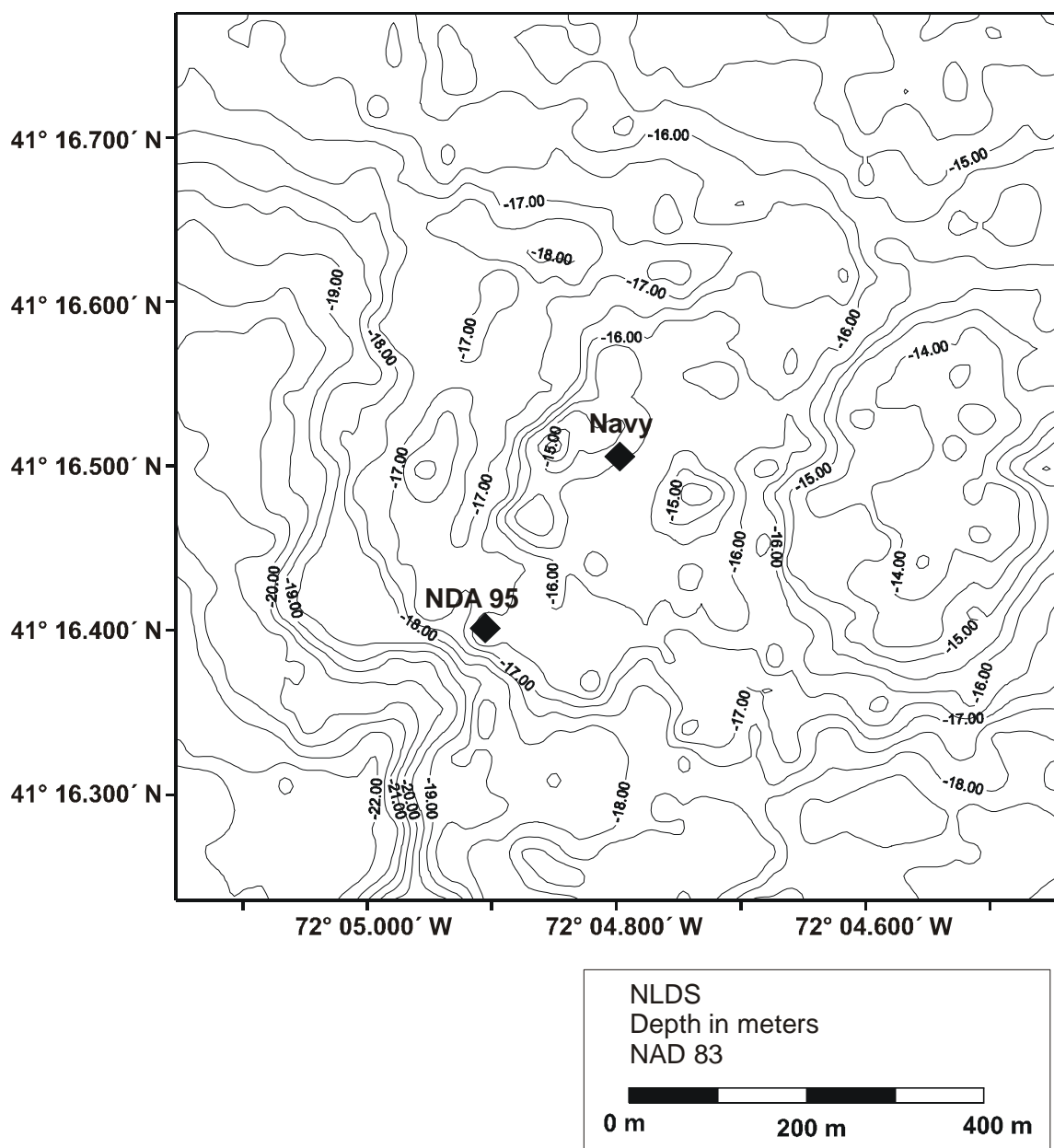
Figure 3-4. Postcap bathymetric survey of the Seawolf Mound area conducted in February 1996 (Gahagan and Bryant)
